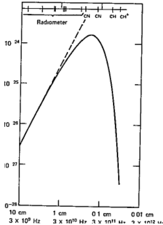
Figure 15.4. Energy density per frequency interval for 2.7°K black-body radiation. The solid curve gives the Planck spectrum (15.5.4); the dashed line gives the Rayleigh–Jeans spectrum (15.5.7) for an antenna temperature of 2.7°K. The short vertical lines mark frequencies at which the black-body temperature has been measured or bounded by radiometer or interstellar absorption observations.
