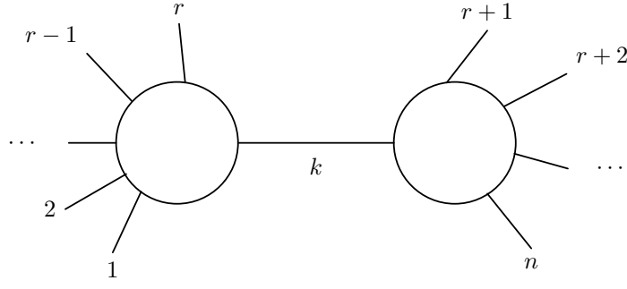
Figure 10.2. A Feynman diagram with the pole structure (10.2.6). Here the line carrying a momentum k represents an elementary particle, one whose field appears in the Lagrangian.
