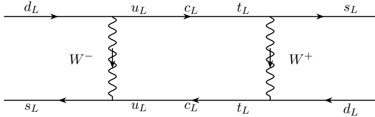
Figure 28.2. A one-loop diagram that can contribute to the \Delta S = 2 effective interaction -(\bar{s} \bar{\sigma}^\mu d)(\bar{d} \bar{\sigma}_\mu s) in both the supersymmetric and non-supersymmetric standard models. Here solid lines are quarks and wavy lines are W^\pm bosons.
