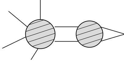
Figure 18.2. A class of Feynman diagrams for the matrix element of the operator \int d^4x \exp(-ip \cdot x) \phi^2(x) that exhibit an ultraviolet divergence. The notation is the same as in Figure 18.1.
