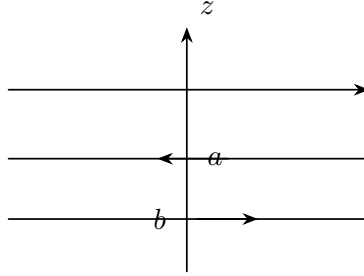
FIGURE 2-1. The contour C in the plane of z = \xi - i\eta .
