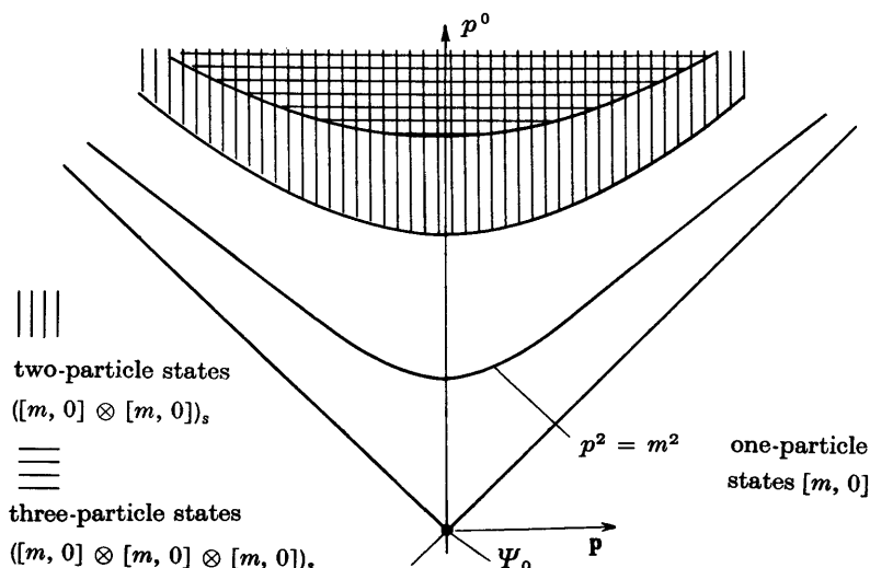
FIGURE 1-3. The spectrum of a theory of neutral scalar mesons of mass m without bound states.
