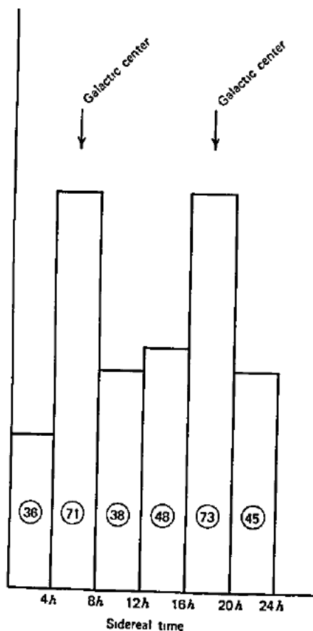
Figure 10.1. Evidence for gravitational radiation emanating from the center of the galaxy. 18 The detector intensity observed by Weber is plotted here (in arbitrary units) against sidereal time. Arrows mark the sidereal times at which the antenna is most nearly perpendicular to the line of sight to the center of the galaxy. Numbers in circles are the observed numbers of coincidences in each time interval.
