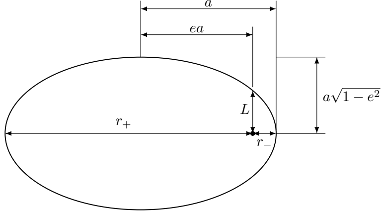
Figure 8.2. Elements of an ellipse referred to in the calculation of the precession of planetary orbits. (The ellipse here has the same eccentricity as the orbit of Icarus.)
