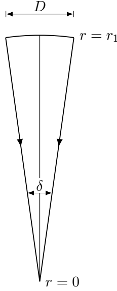
Figure 14.2. Quantities used in the calculation of angular diameters and proper motions. The angle \delta is greatly exaggerated.
