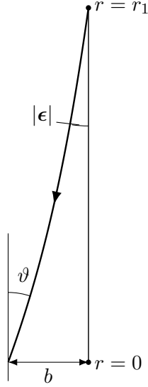
Figure 14.1. Quantities used in the calculation of parallaxes and apparent luminosities. The angles and the curvature of the light ray are greatly exaggerated.
