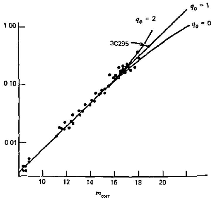
Figure 14.12. Red shifts and corrected apparent magnitudes for 42 first-ranked cluster galaxies. Data are taken from a 1970 review of Sandage. 44 Curves represent fits of Eq. (14.6.10) to the data.
