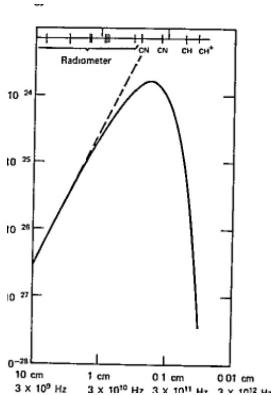
Figure 15.4. Energy density per frequency interval for 2.7°K black-body radiation. The solid curve gives the Planck spectrum (15.5.4); the dashed line gives the Rayleigh–Jeans spectrum (15.5.7) for an antenna temperature of 2.7°K. The short vertical lines mark frequencies at which the black-body temperature has been measured or bounded by radiometer or interstellar absorption observations.
