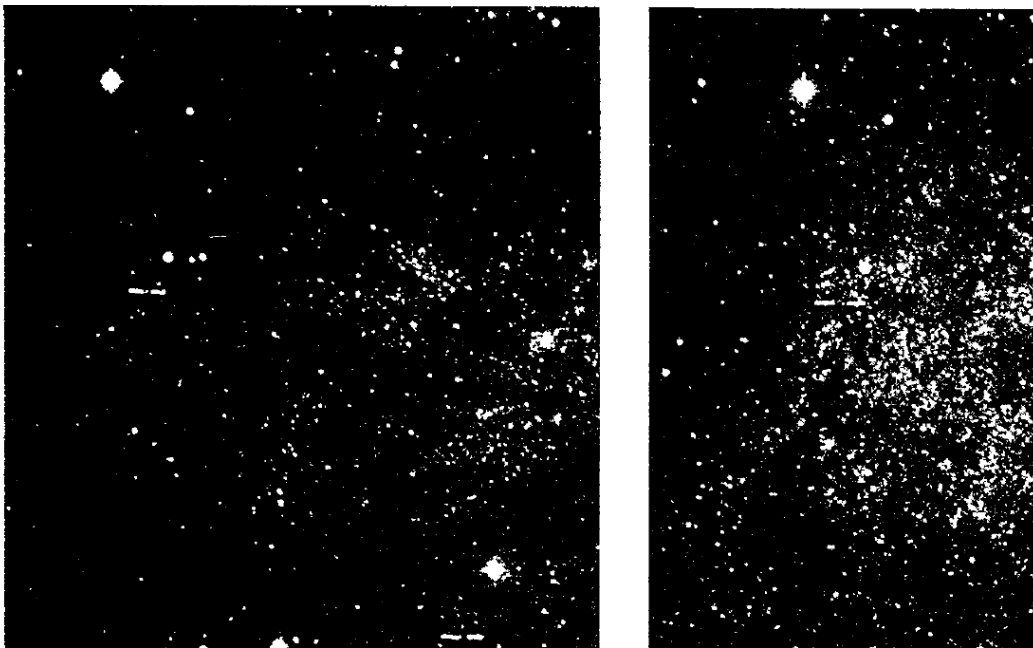
Figure 14.9. Variable stars in a portion of M31. Two of the variables are marked. This photograph was taken with the 200-in. telescope at Mt. Palomar. (Courtesy Mt. Wilson and Mt. Palomar observatories.)
