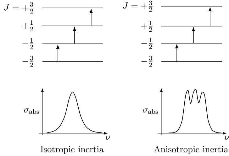
Figure 3.1. The \text{Li}^7 absorption spectrum as a test of the isotropy of inertia (frequency differences and line splitting greatly exaggerated).
