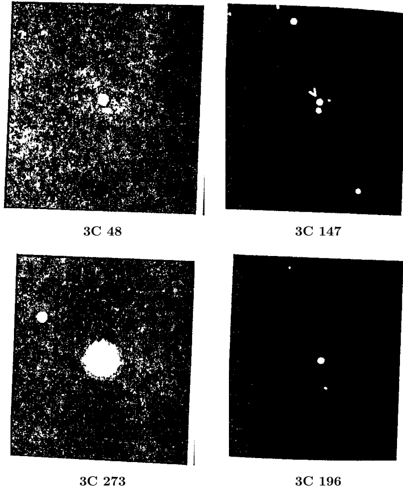
Figure 11.1. Four quasi-stellar objects. These photographs were taken with the 200-in. telescope at Mt. Palomar, following position determinations by radio astronomers. (Courtesy Mt. Wilson and Palomar Observatories.)
