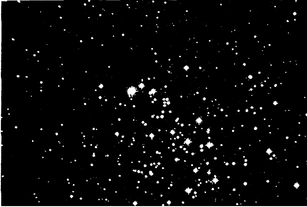
Figure 14.5. The open cluster NGC 2682, in Cancer, photographed with the 200-in. telescope at Mt. Palomar. (Courtesy Mt. Wilson and Mt. Palomar observatories.)
