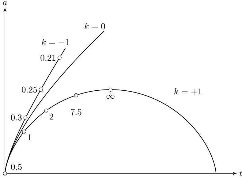
Figure 15.1. Solutions of Einstein's equations for a Robertson-Walker universe with curvature k = +1 , k = 0 , and k = -1 . The numbers along the curves k = \pm 1 give the values of the deceleration parameter q at various epochs.
