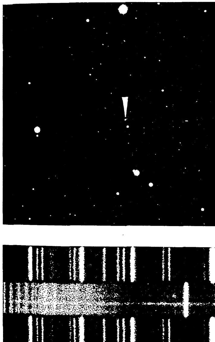
Figure 14.11. The radio galaxy 3C295 in Boötes. The spectrum of this galaxy, shown below, reveals a red shift z = 0.46 , the largest yet observed for any galaxy. This photograph and spectrograph were taken with the 200-in. telescope at Mt. Palomar. (Courtesy Mt. Wilson and Mt. Palomar observatories.)
