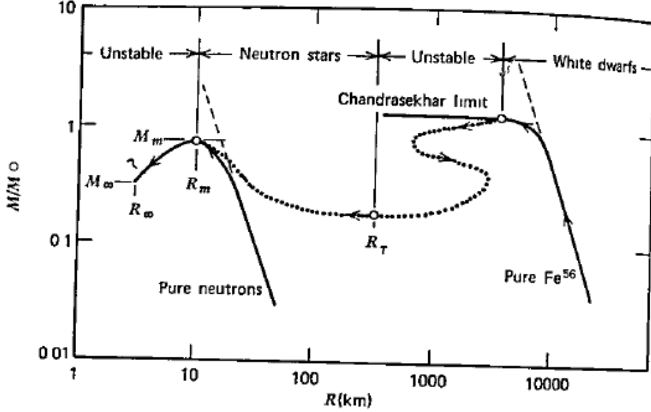
Figure 11.2. Configurations of stellar equilibrium. The solid curves on the left and right represent the Oppenheimer–Volkoff 10 solution for a pure neutron star and the Chandrasekhar 8 solution for a pure \text{Fe}^{56} white-dwarf star, respectively. The dashed lines give the extrapolated nonrelativistic solutions in these two cases. The dotted line represents the interpolating solution of Harrison, Thorne, Wakano, and Wheeler, 12 which takes into account the shift in chemical composition from \text{Fe}^{56} to neutrons. Arrows indicate the direction of increasing central density. As shown in Theorem 1, the various transitions between stability and instability occur at the maxima and minima of M , marked here with small circles.
