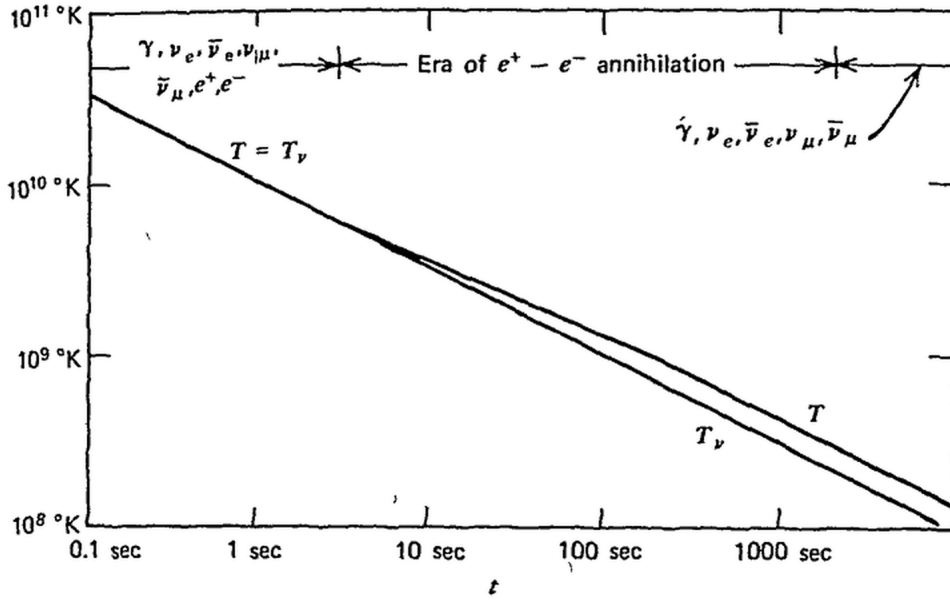
Figure 15.5. Thermal history of the early universe. Here T is the temperature of the \gamma - e^+ - e^- plasma, and T_\nu is the temperature of the decoupled \nu_e, \bar{\nu}_e, \nu_\mu, \bar{\nu}_\mu .
