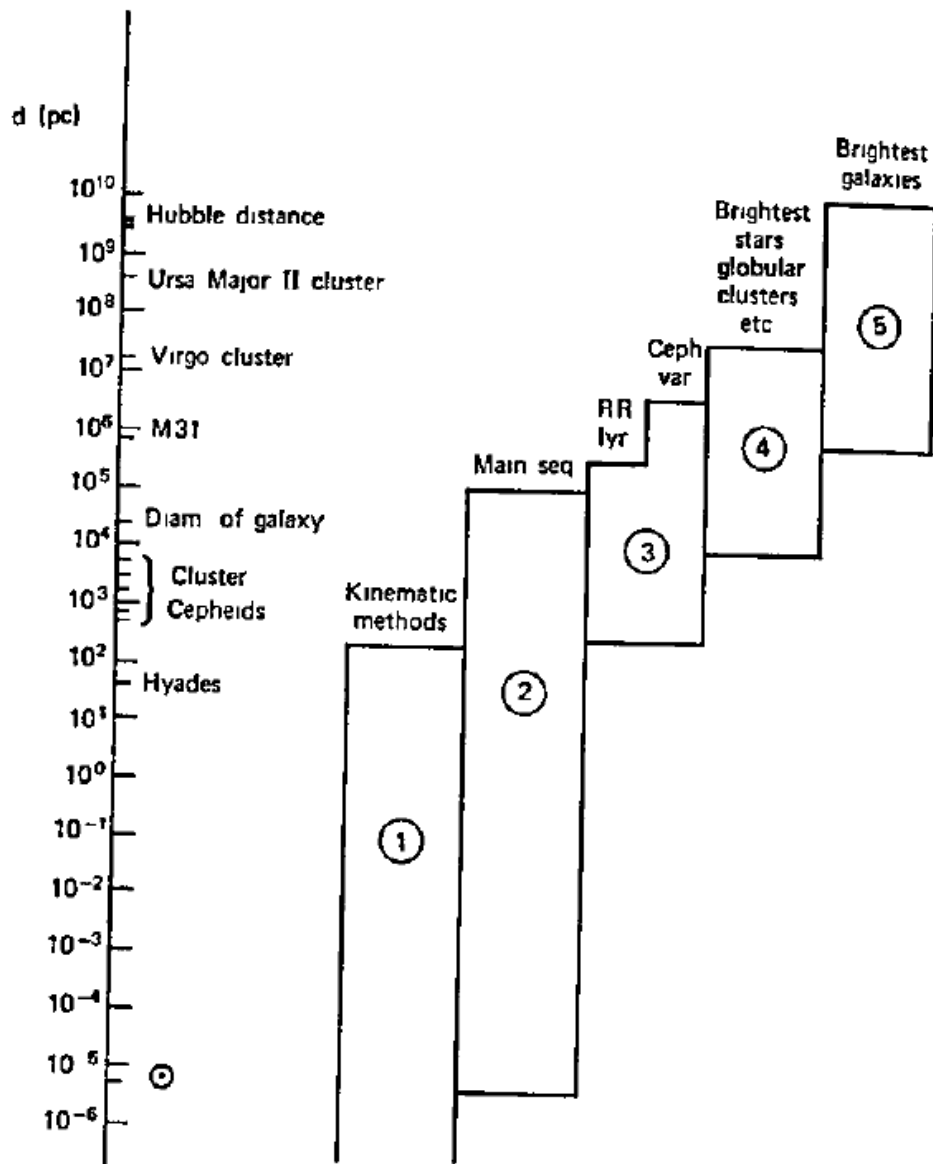
Figure 14.3. The cosmic distance ladder. The position and height of the vertical bars mark roughly the range of distance over which each class of distance indicator may be used.
