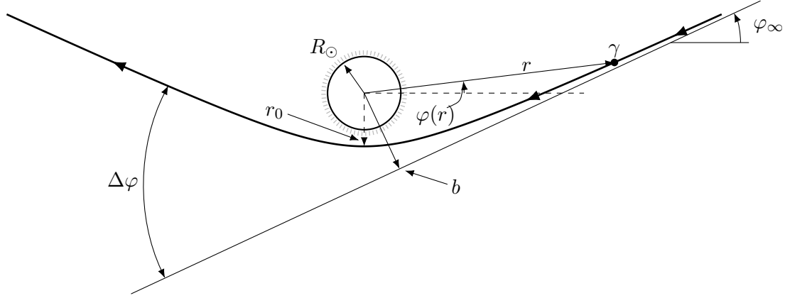
Figure 8.1. Quantities referred to in the calculation of the deflection of light by the sun. (Deflection greatly exaggerated.)
