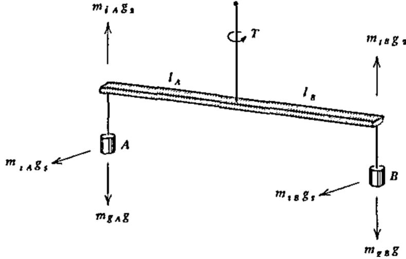
Figure 1.2. Schematic view of the Eötvös experiment.
