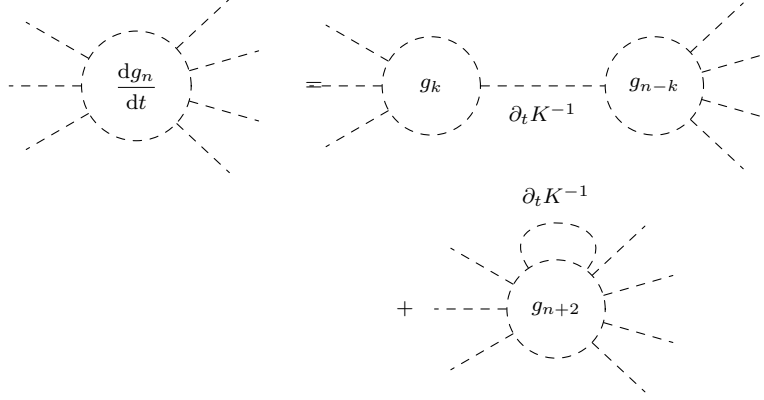
Figure 9.2. The RG equation.
