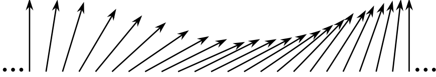
Figure 7.2. A Nambu–Goldstone excitation.
