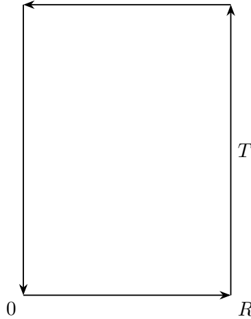
Figure 8.3. The Wilson loop for the static potential.
