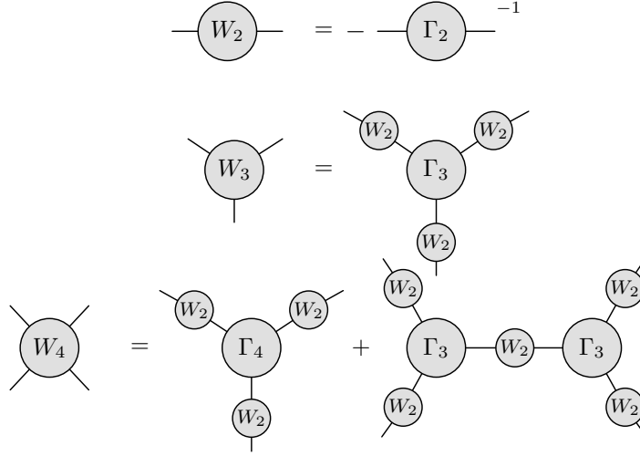
Figure 3.1. Legendre transform W[J] = \Gamma[\phi] + \int d^D x \phi J makes trees.
