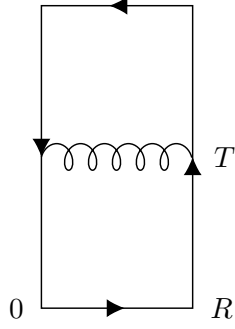
Figure 9.8. Wilson loop for the static potential.
