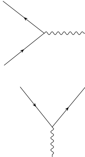
Figure 1.2. Scattering in one frame is production amplitude in another.
