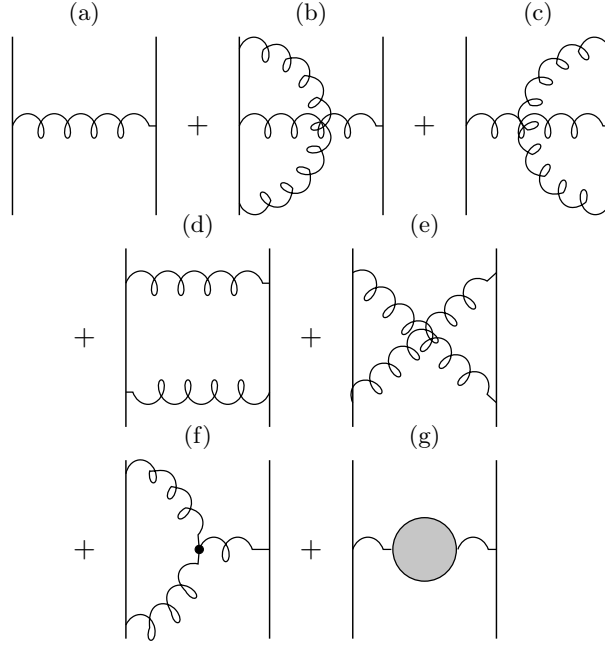
Figure 9.9. One-loop contributions to the potential.
