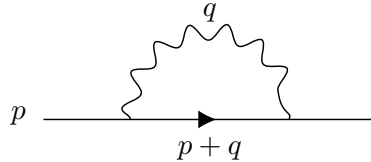
Figure 9.7. One-loop self-energy in QED.
