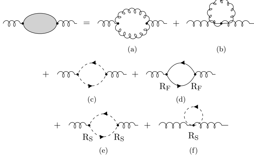
Figure 9.10. One-loop contributions to gluon vacuum polarization.
