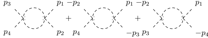
Figure 9.4. s-, t- and u-channel diagrams for the one-loop four-point function.
