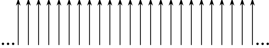
Figure 7.1. A state with spontaneously broken symmetry.
