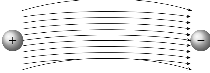
Figure 8.2. A flux tube between monopoles in a superconductor.
