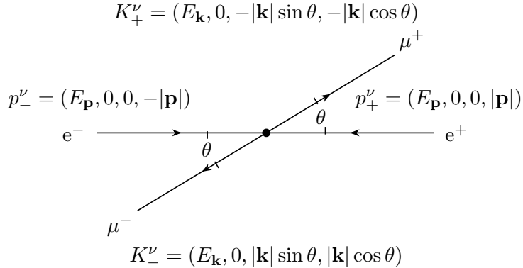
Figure 6.3. \mu^+, \mu^- pair production by annihilation of massless e^+, e^- in the center-of-mass frame.
