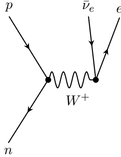
Figure 8.1. Fermi’s theory of weak interactions.
