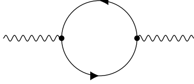
Figure 9.6. Vacuum polarization in QED.
