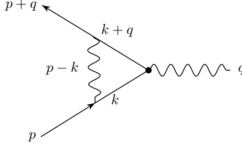
Figure 6.4. One-loop vertex correction.
