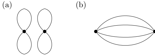
Figure 9.1. Examples of divergent diagrams.
