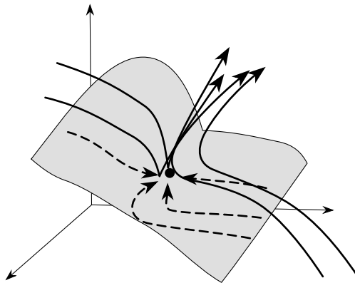
Figure 9.3. Renormalization-group trajectories near a critical surface.
