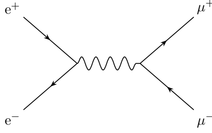
Figure 6.2. Heavy-fermion production in e^+, e^- annihilation.
