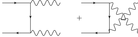
Figure 6.1. Gauge-boson production in e^+, e^- annihilation.
