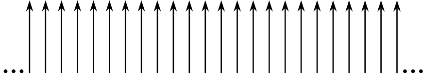
Figure 7.1. A state with spontaneously broken symmetry.
