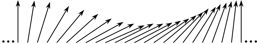
Figure 7.2. A Nambu–Goldstone excitation.
