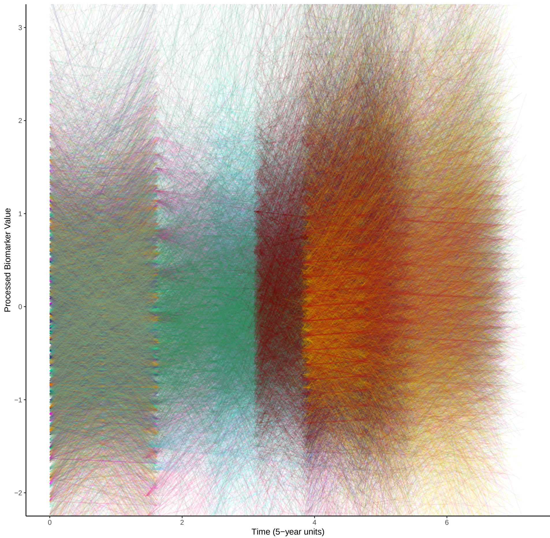
Longitudinal Biomarker Measurement in the Framingham Heart Study
