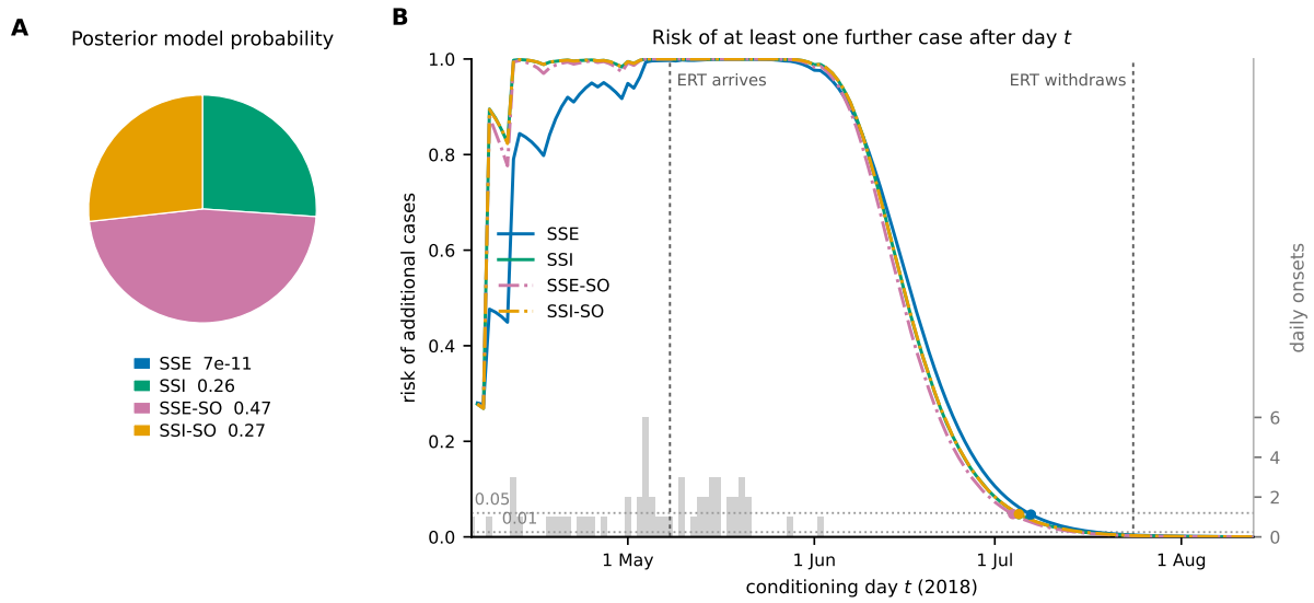
Figure S5: No switchpoint, with R and k fixed. The four models of Fig. 4 with R held at one value throughout and k at its literature value, so that only the latent states are estimated. A : posterior model probabilities under a uniform prior over the four models; SSE, with nothing to integrate over, contributes its likelihood exactly. B : RAC, with filled circles where each curve settles below 0.05. The onset-anchored models are dash-dotted because, with the switch removed, their curves lie close enough to the infection-anchored ones to hide them. With R constant the reset to R_{\text{pre}} is a no-op, so these are forward posterior predictives (Section 6.6).
