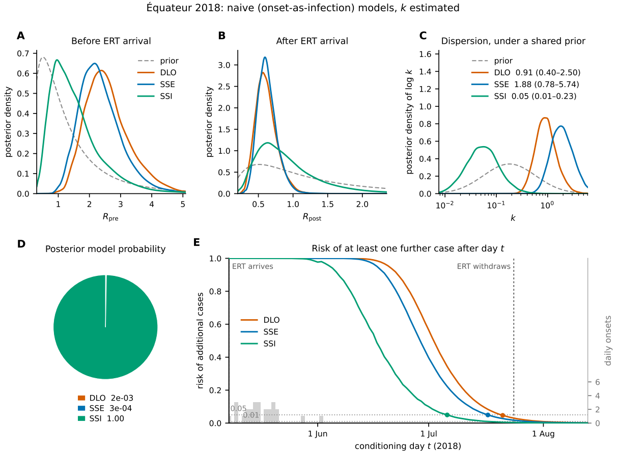
Figure 3: The models infer different dispersion parameters, and their risk curves remain separated. As Fig. 2, with k estimated. C : the three k posteriors over the prior they share, with each model's posterior median and 95% credible interval in the legend. D : posterior model probabilities. E : risk of additional cases, with the view starting at the ERT's arrival because from there until well past the last case all three curves sit at 1. The curves are computed over the whole window either way; only the view is trimmed.
