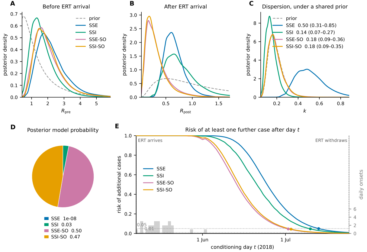
Figure S2: Onset anchoring with the dispersion estimated. The four models of Fig. 4, with k given the shared prior drawn in panel C instead of being held at its literature value; panels as in Fig. 3. In panel C, SSE-SO's k posterior shifts below SSE's and onto the prior's median, whereas SSI-SO remains close to SSI. This contrast supports attenuation of day-level, but not individual-level, heterogeneity when onsets are treated as infections. The risk curves in panel E are separated much as they are at fixed k .
