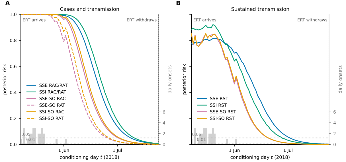
Figure 5: Onset anchoring brings the decline forward whichever risk is asked about. Models fitted with k fixed at 0.18. A: RAC (solid) and RAT (dashed) for all four models. Under infection anchoring a case is a transmission event, so RAC = RAT by construction and SSE and SSI each have a single solid curve; only SSE-SO and SSI-SO separate the two. B: RST for all four models, drawn solid since it is the only risk in the panel. Colours identify models in both panels. Grey bars show daily symptom onsets; vertical lines mark ERT arrival and withdrawal, and horizontal lines mark the 0.05 and 0.01 decision thresholds. Each point is a separate posterior fit to the record through that conditioning day, followed by a reset to R_{\text{pre}} . DLO is omitted because its day-level negative-binomial variation does not define individual transmission lineages.
