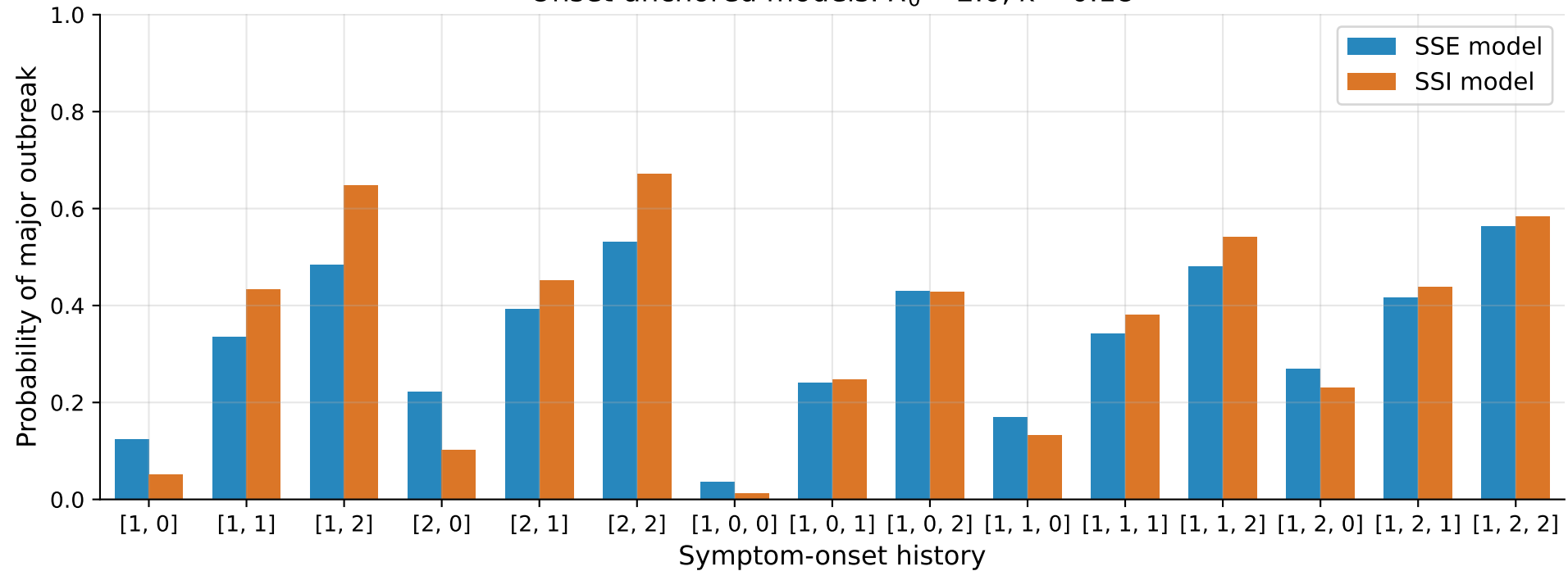
Onset-anchored models: R_0 = 2.0 , k = 0.18
