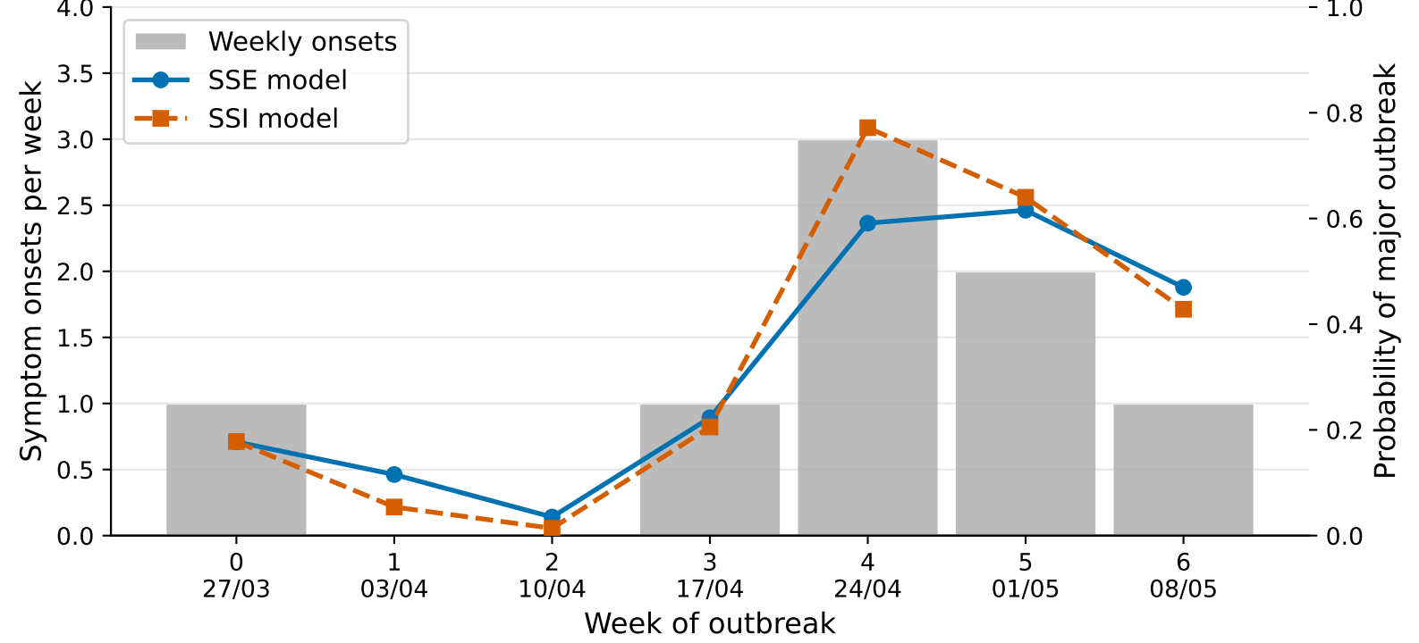
2017 Likati EVD outbreak: real-time PMO ( R_0 = 2.0 , k = 0.18 , threshold: peak weekly onsets \geq 100 )
