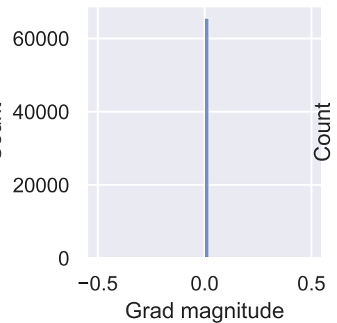
layers.4.weight
