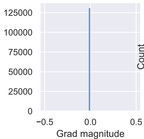
layers.2.weight
