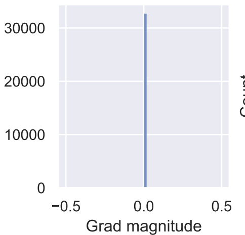
layers.6.weight
