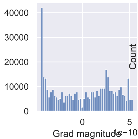
layers.0.weight
