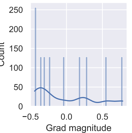
layers.8.weight
