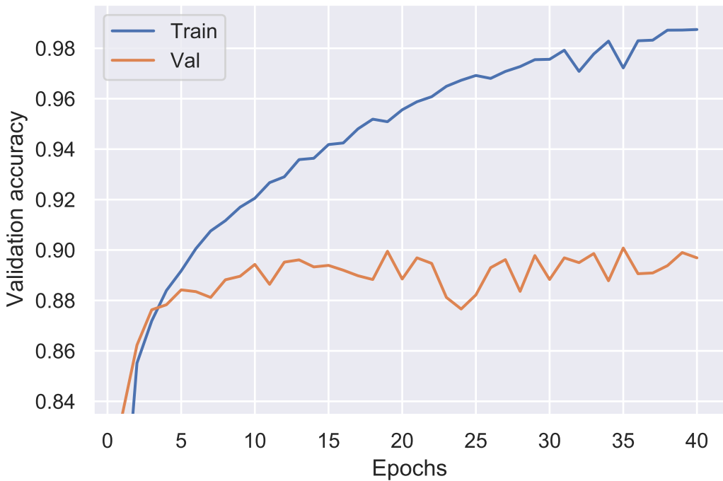
Validation performance of FashionMNIST_SGD
