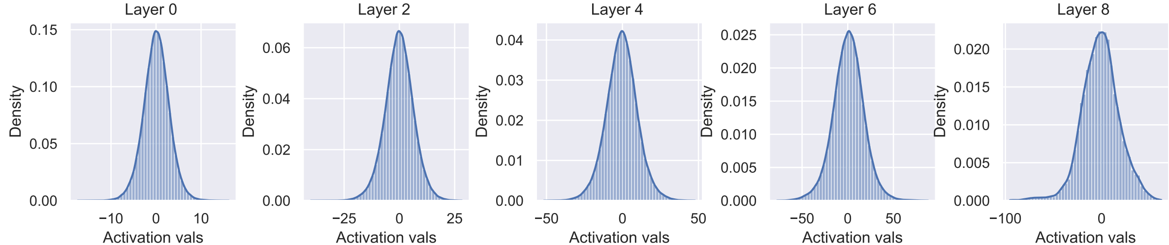
Activation distribution
