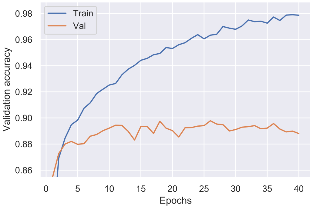
Validation performance of FashionMNIST_Adam
