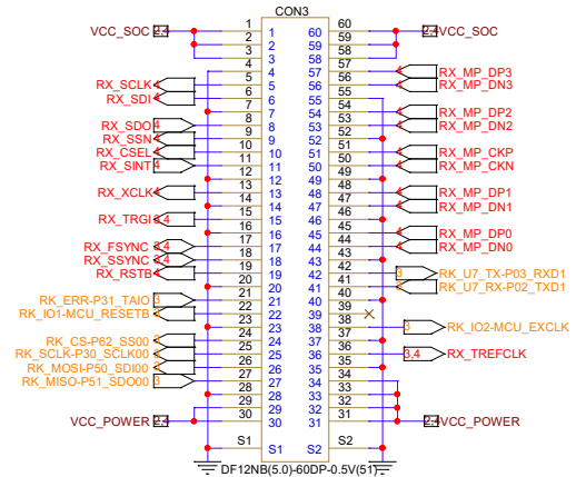
SOC Board Connect
