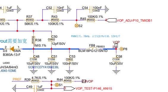
VOP可调: -19.6V ~ -32.5V
