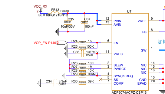
Power Inverting Regulator
