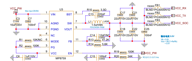
DC Buck 12V to 5.0V
