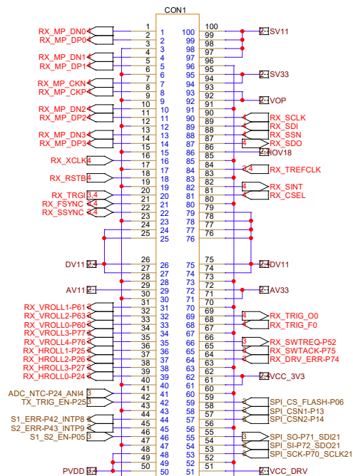
RX_TX MiniModule Connect
