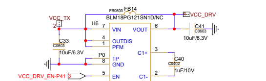
DC Boost 5V
