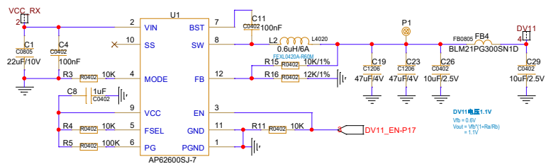
DC Buck DV11 1.1V
