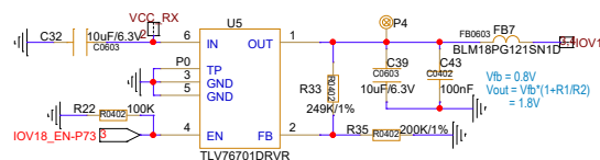
LDO IOV18 1.8V
