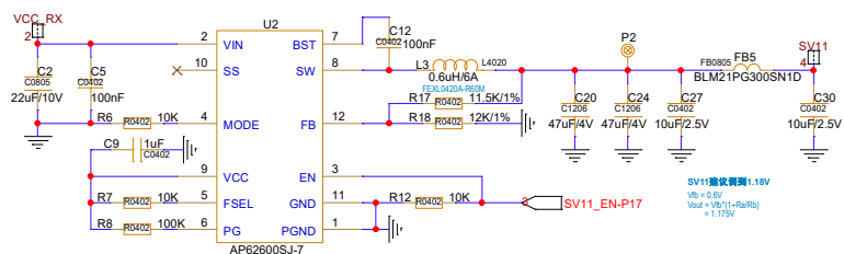
DC Buck SV11 1.18V
