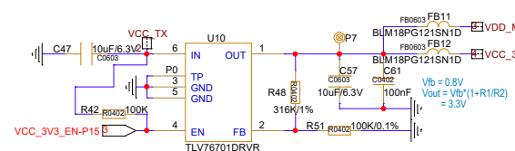
LDO VCC_3V3 3.3V
