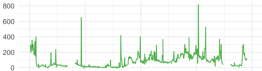
\text{NO}_2 / pptv
