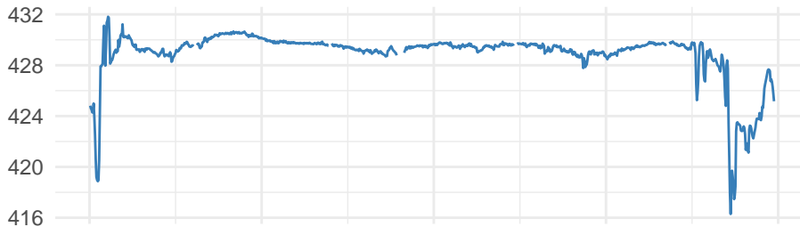
NO / pptv
