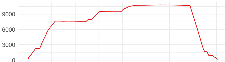
\text{CO}_2 / ppmv
