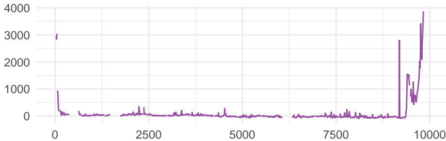
NO 2 / pptv
