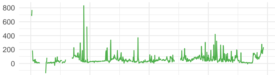
NO 2 / pptv
