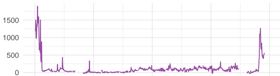
\text{NO}_2 / pptv
