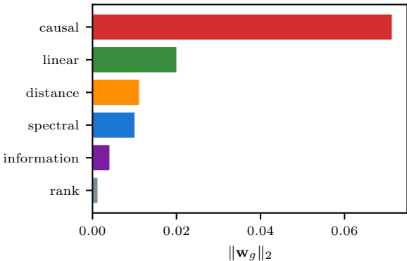
Statistical signature
