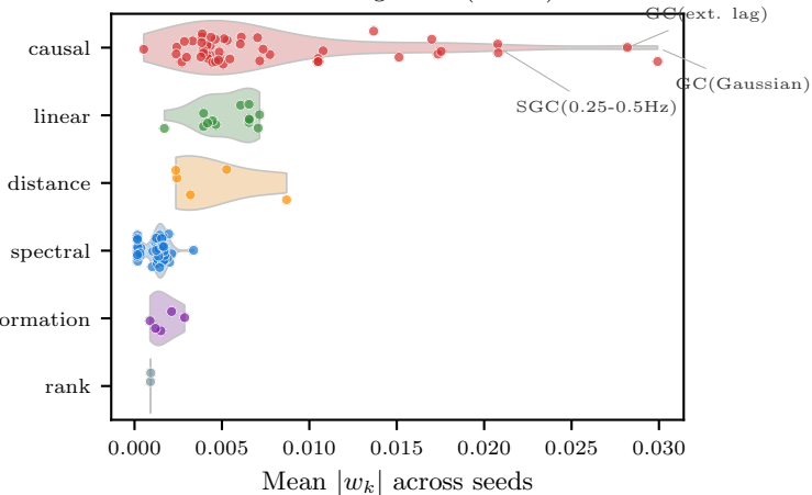
Statistical signature ( n=500 )
