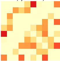
MI (Gaussian) (symmetric)
