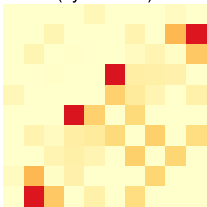
Covariance (symmetric)
