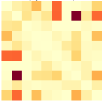
SGC (0.25–0.5 Hz) (directed)
