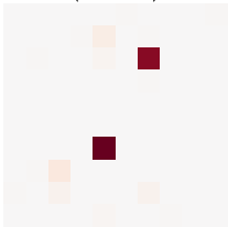
GC (Gaussian) (directed)
