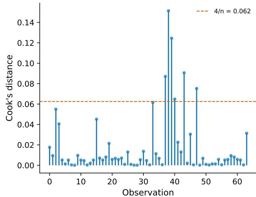
H1: Cook's Distance
