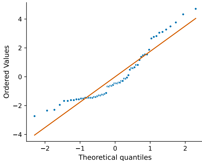
H1: Q-Q Plot
