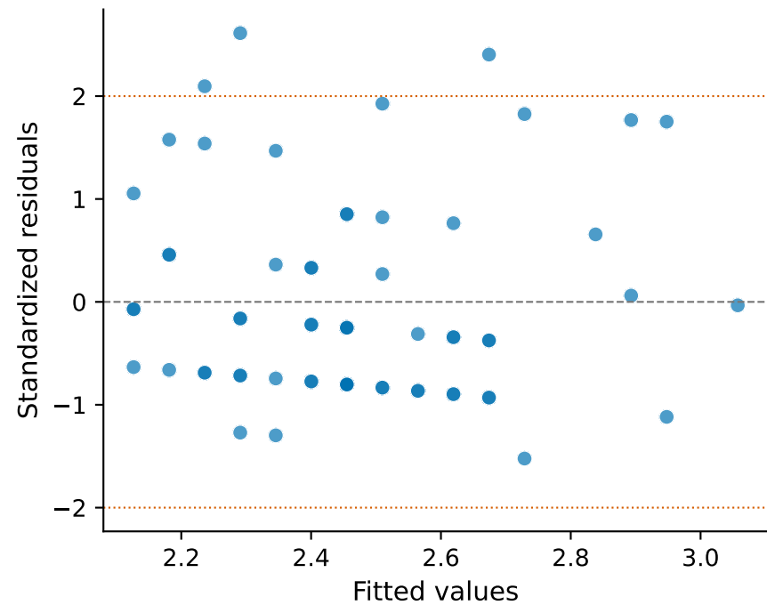
H1: Residuals vs Fitted
