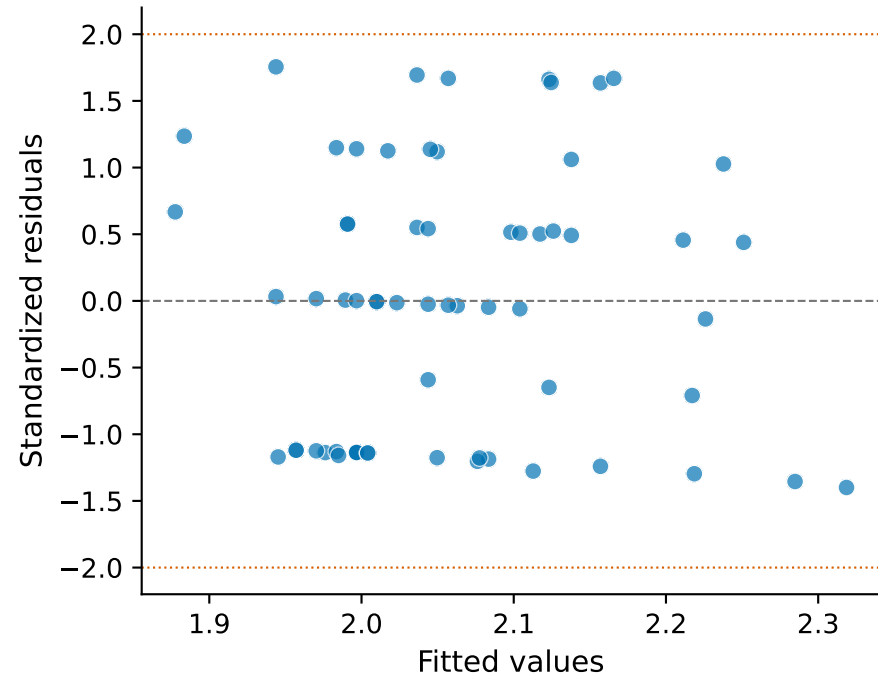
H3: Residuals vs Fitted
