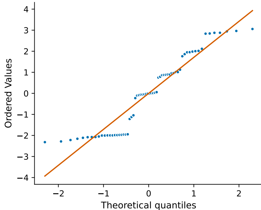
H3: Q-Q Plot
