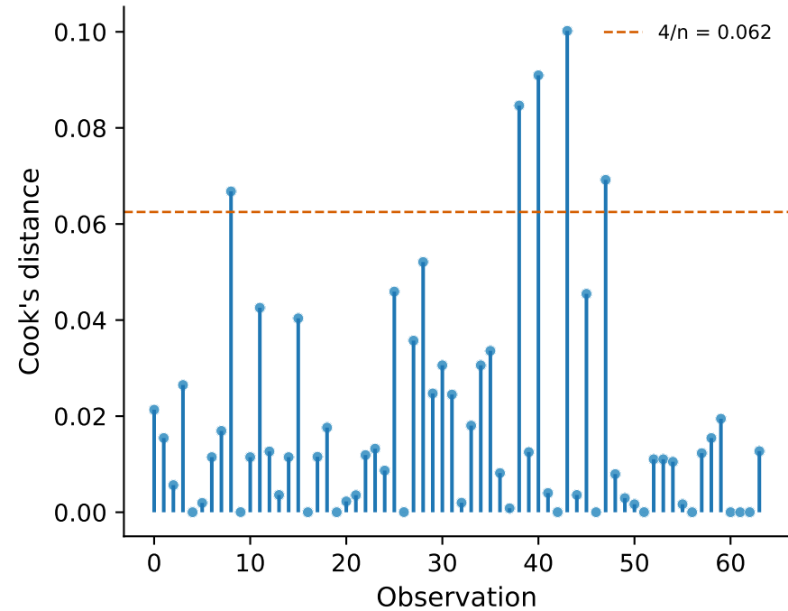
H3: Cook's Distance
