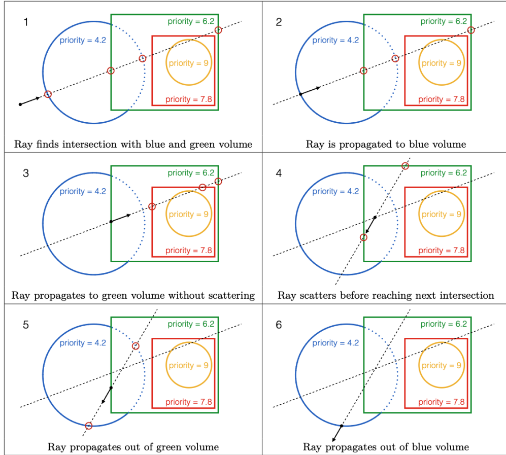
Figure B.2.: Illustration of the Union propagation algorithm for a single scattering event between two overlapping volumes. Only intersections actually relevant given the ray's current volume are calculated at each step (the orange volume, never reachable from the ray's actual path here, is never tested).
