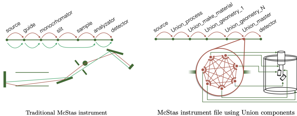
Figure B.1.: Left: the linear succession of components in a traditional McStas instrument file. Right: the same instrument using Union components – all ray tracing for the sample environment happens inside a single master component, which works around the normal McStas component sequence to achieve native multiple scattering between an arbitrary number of volumes.
