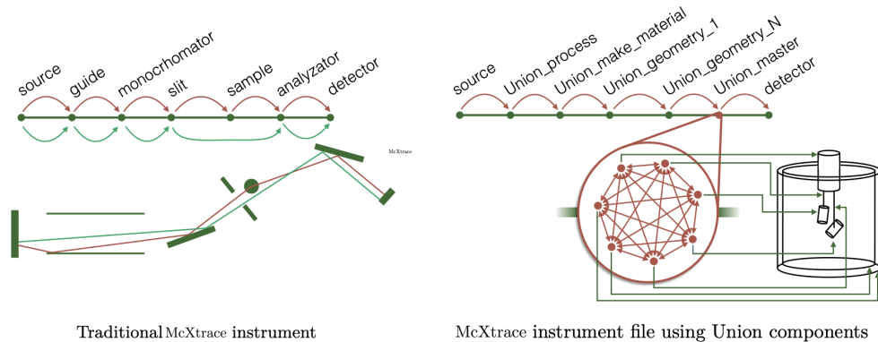
Figure A.1.: Left: the linear succession of components in a traditional McXtrace instrument file. Right: the same instrument using Union components – all ray tracing for the sample environment happens inside a single master component, which works around the normal McXtrace component sequence to achieve native multiple scattering between an arbitrary number of volumes. (Originally illustrated for McStas; the same principle applies unchanged to McXtrace.)
