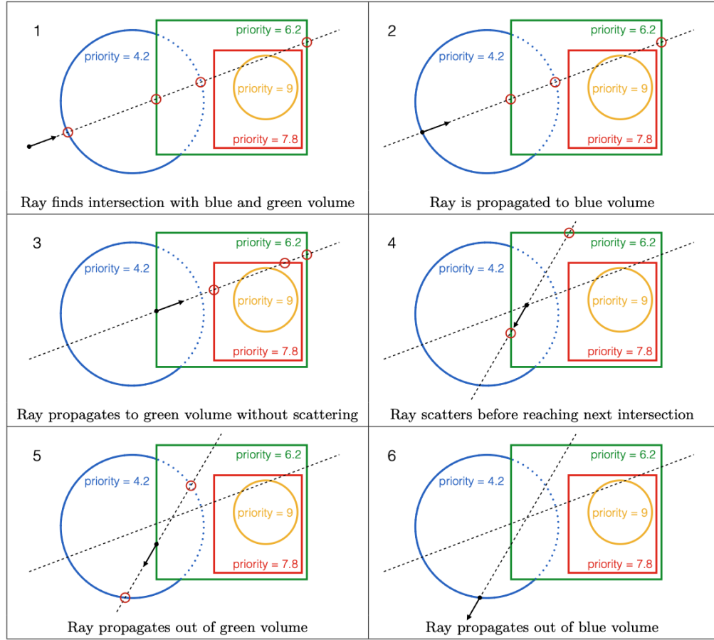
Figure A.2.: Illustration of the Union propagation algorithm for a single scattering event between two overlapping volumes. Only intersections actually relevant given the ray's current volume are calculated at each step (the orange volume, never reachable from the ray's actual path here, is never tested).
