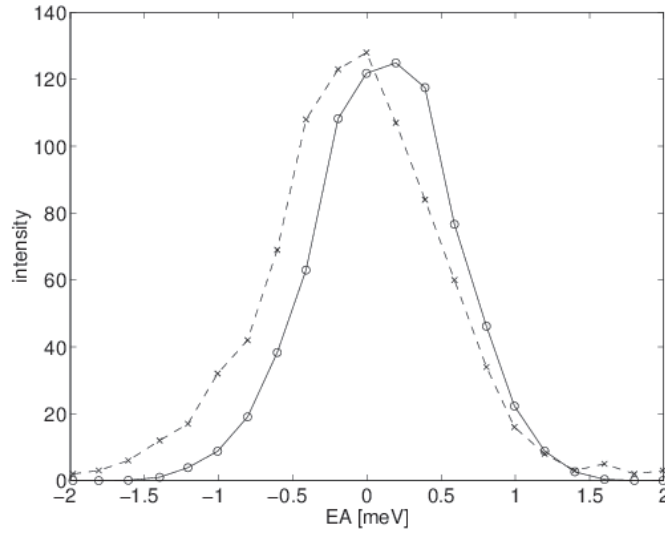
Figure 9.7.: TAS1: Scans of the analyser energy on a V-sample. Collimations: open-30'-28'-67'. "x": measurements, "o": simulations.
