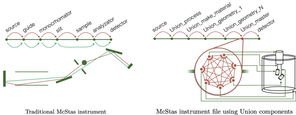
Figure 6.1.: Left: the linear succession of components in a traditional McStas instrument file. Right: the same instrument using Union components – all ray tracing for the sample environment happens inside a single master component, which works around the normal McStas component sequence to achieve native multiple scattering between an arbitrary number of volumes.
