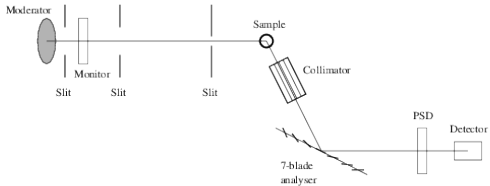
Figure 9.8.: A sketch of the PRISMA instrument.
