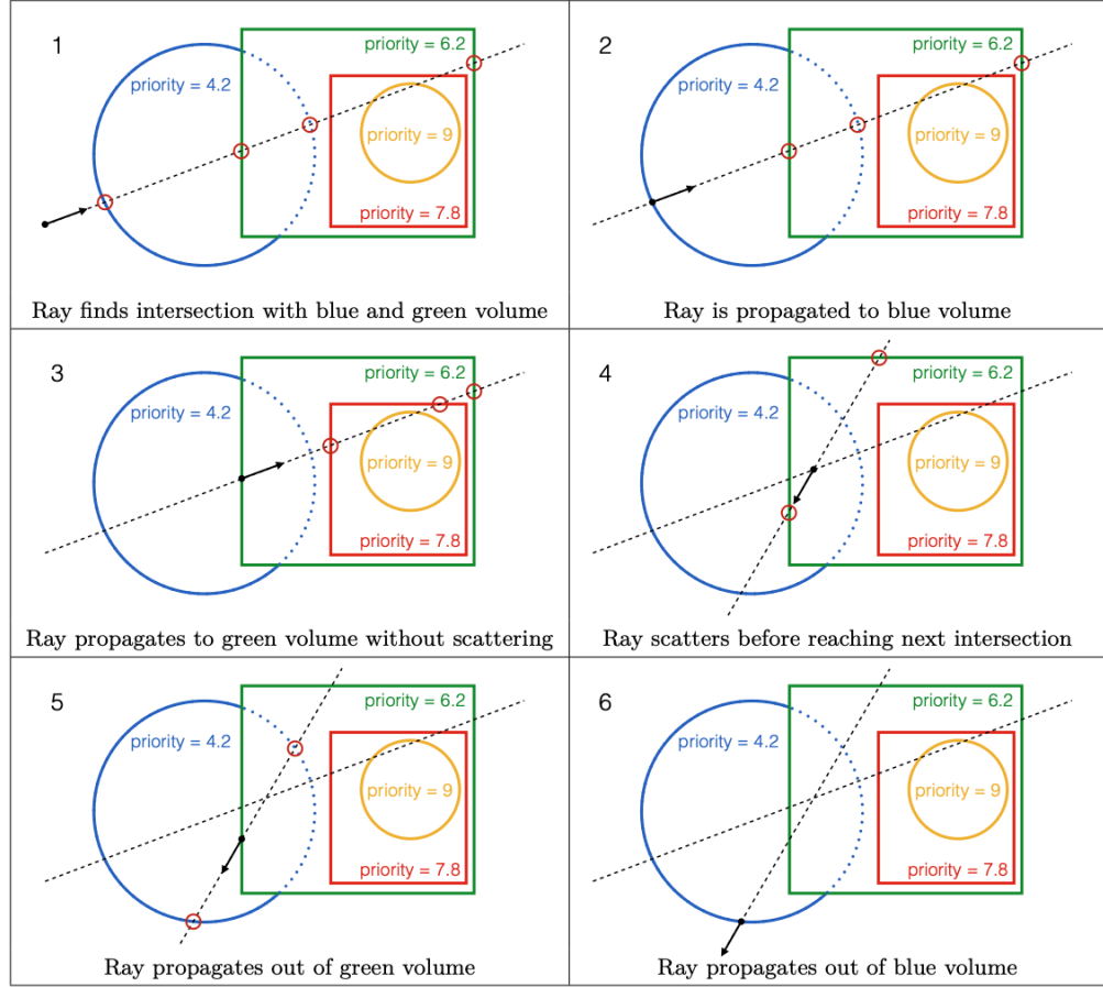
Figure 6.2.: Illustration of the Union propagation algorithm for a single scattering event between two overlapping volumes. Only intersections actually relevant given the ray's current volume are calculated at each step (the orange volume, never reachable from the ray's actual path here, is never tested).
