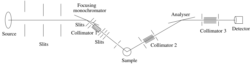
Figure 9.3.: A sketch of the TAS1 instrument.
