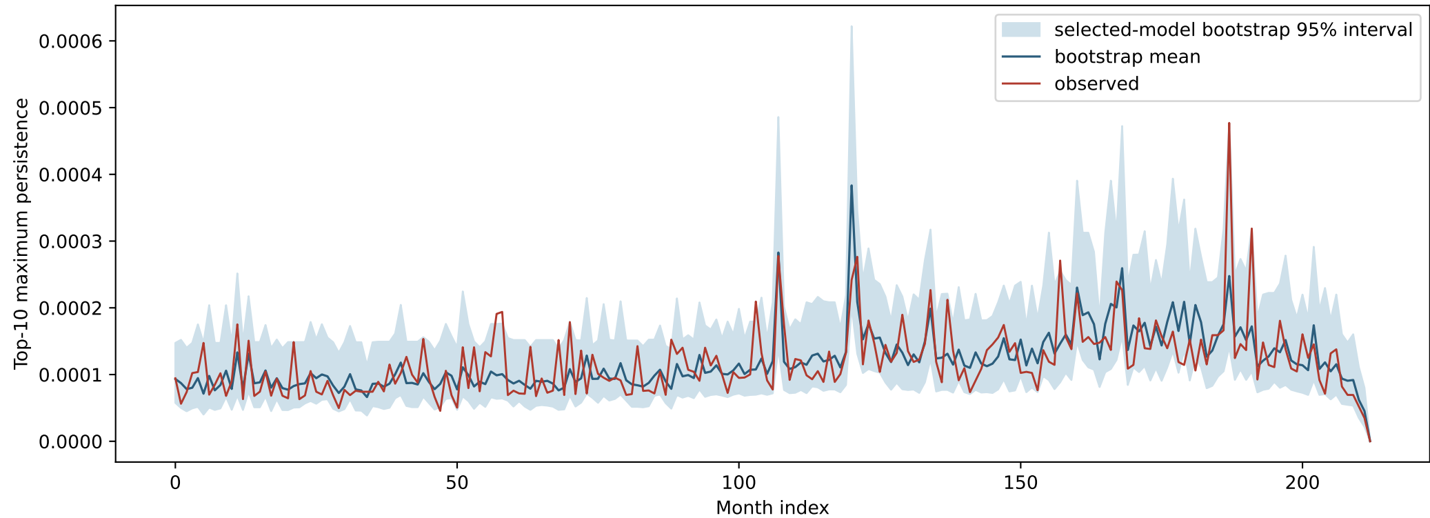
Monthly maximum H_1 persistence with selected-model bootstrap interval
