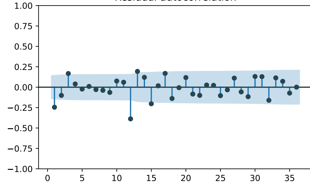
Residual autocorrelation
