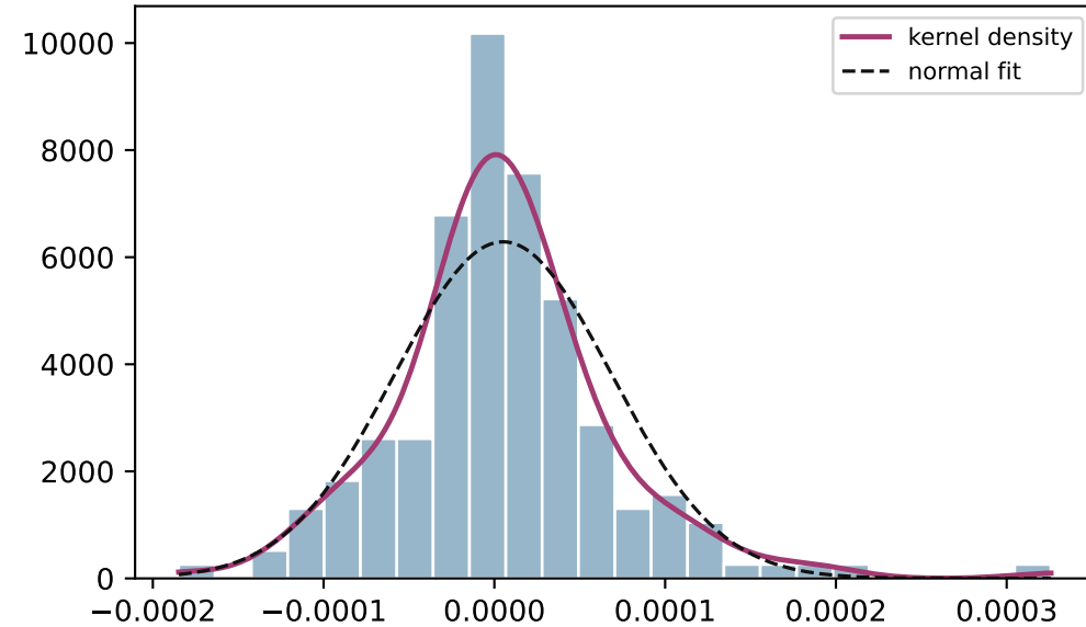
Histogram and density
