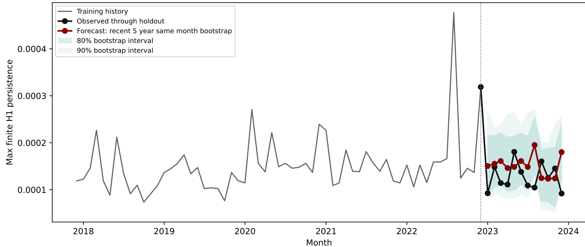
Maximum finite H1 persistence, 2023 holdout Selected forecast: recent 5 year same month bootstrap
