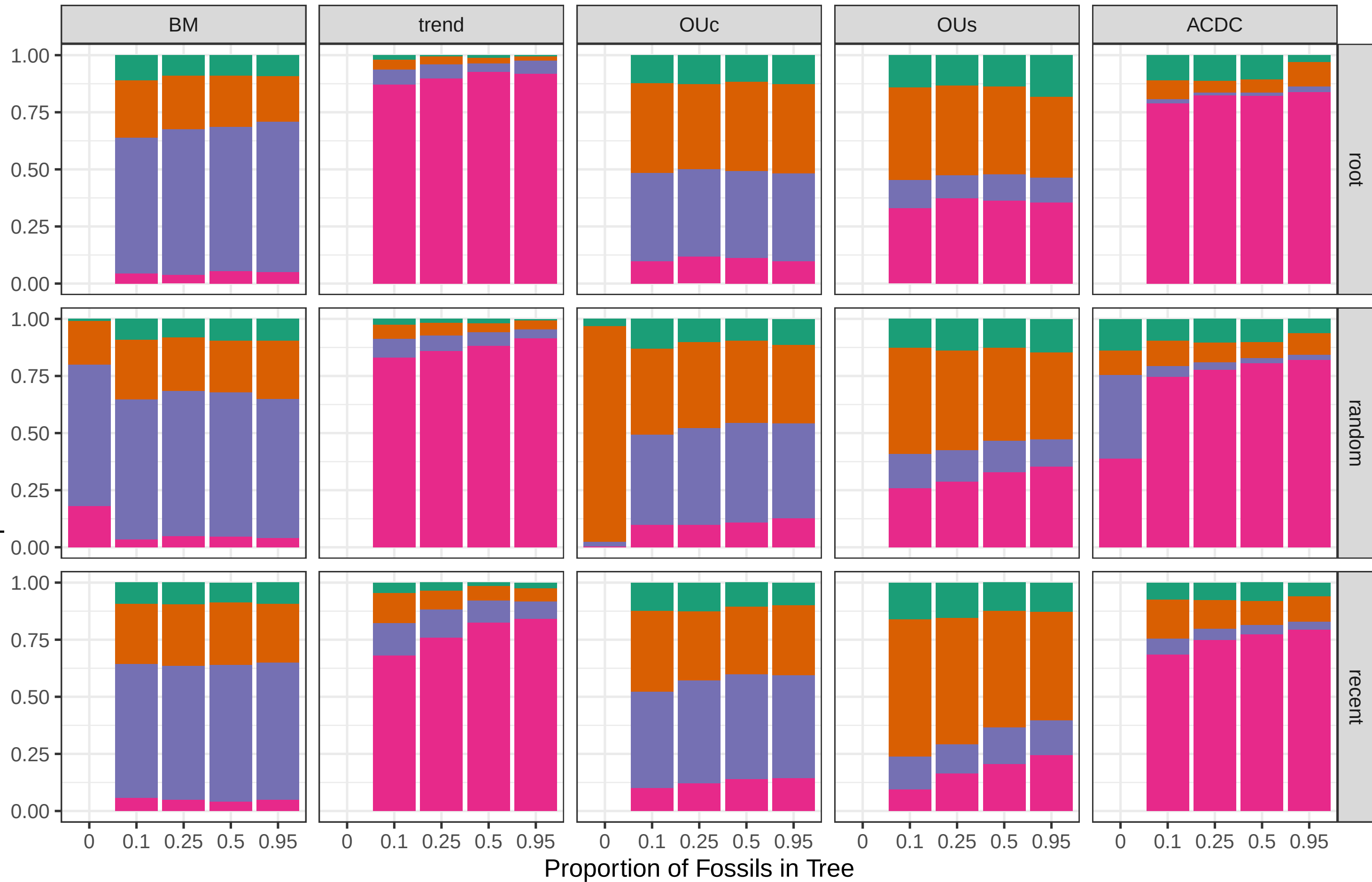
Fit Status
