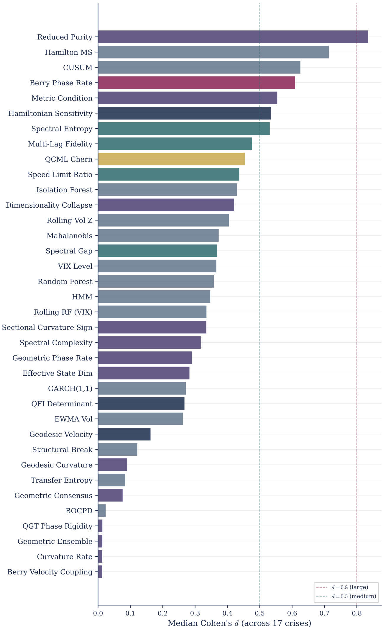
Regime Detection: All Methods Ranked by Median Cohen's d
