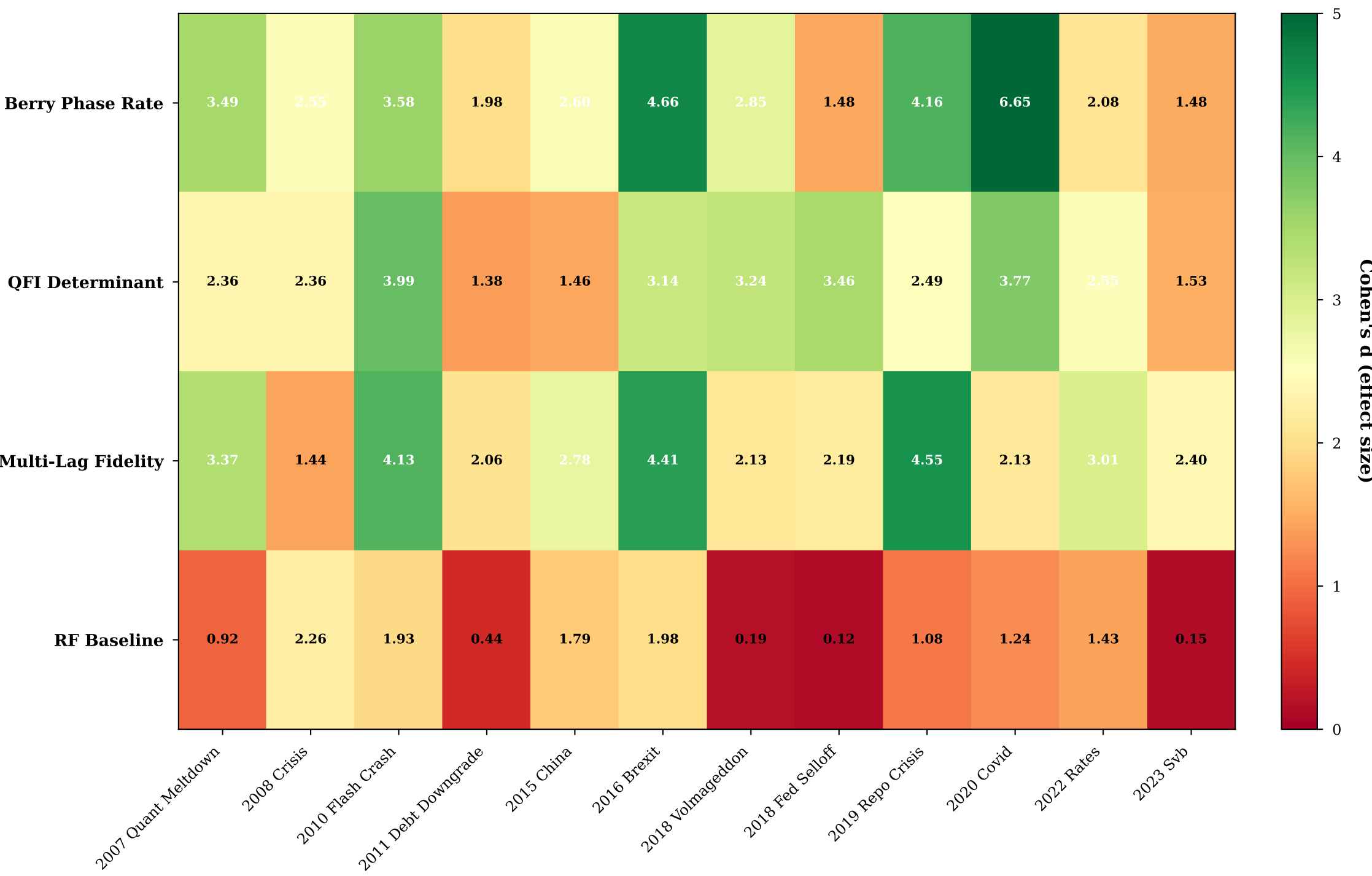
Per-Crisis Performance Heatmap (Best QCML Condition vs RF)
