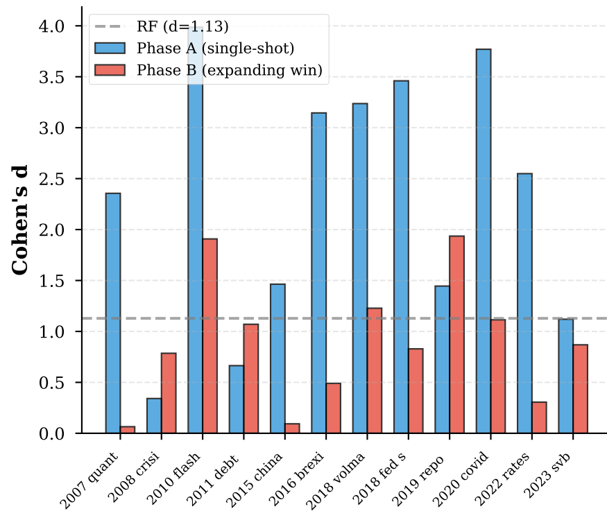
QFI Determinant (Phase A: d=2.29 , Phase B: d=0.89 )
