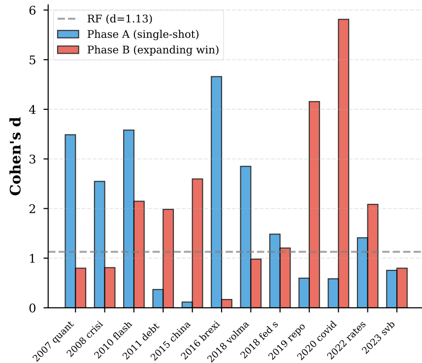
Berry Phase Rate (Phase A: d=1.87 , Phase B: d=1.96 )
