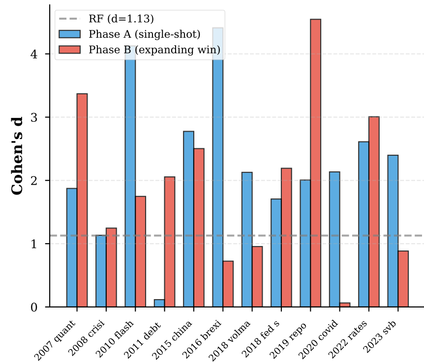
Multi-Lag Fidelity (Phase A: d=2.28 , Phase B: d=1.94 )
