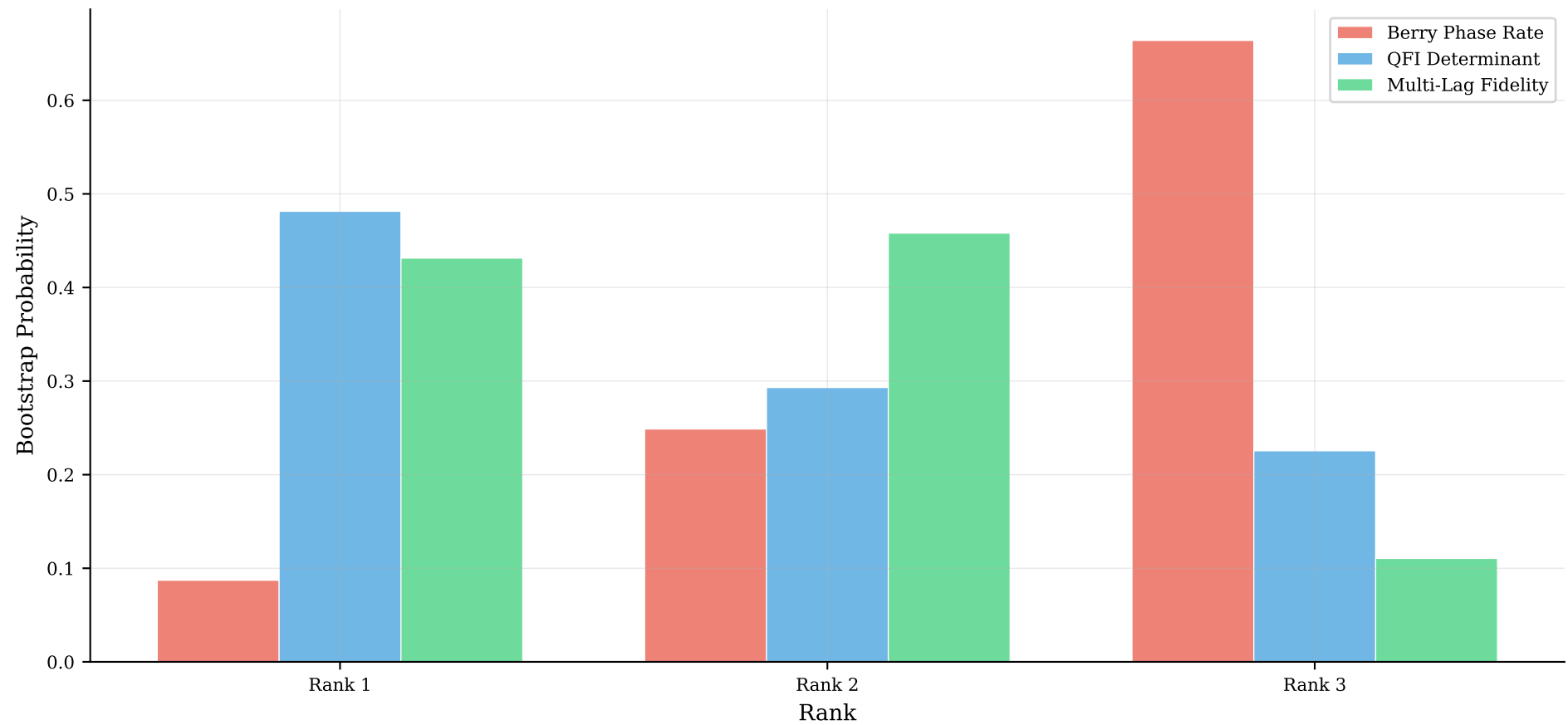
Bootstrap Ranking Distribution ( n = 10,000 )
