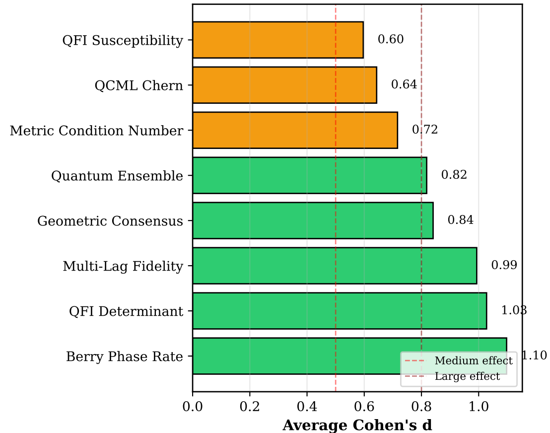
Average Effect Size Across Crises
