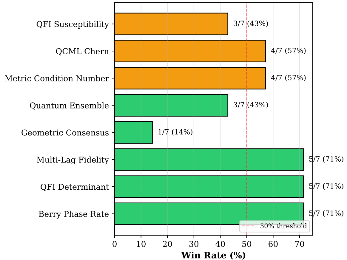
Success Rate ( p < 0.05 , d > 0.5 )
