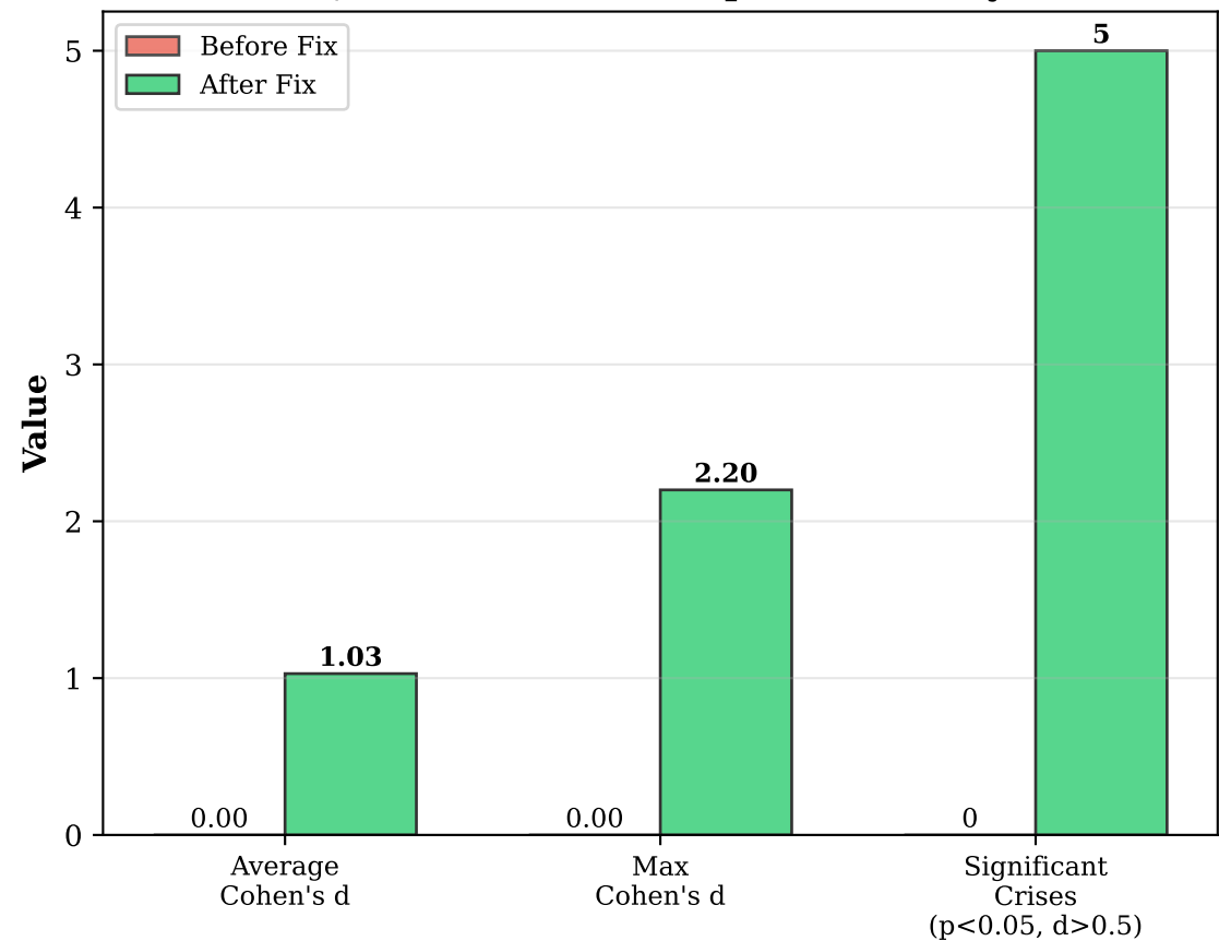
QFI Determinant: Impact Summary
