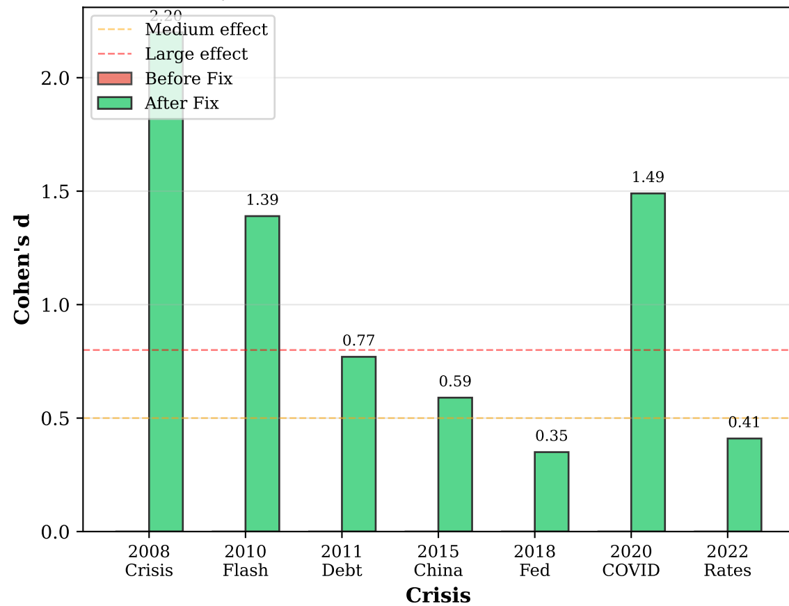
QFI Determinant: Before vs After Fix
