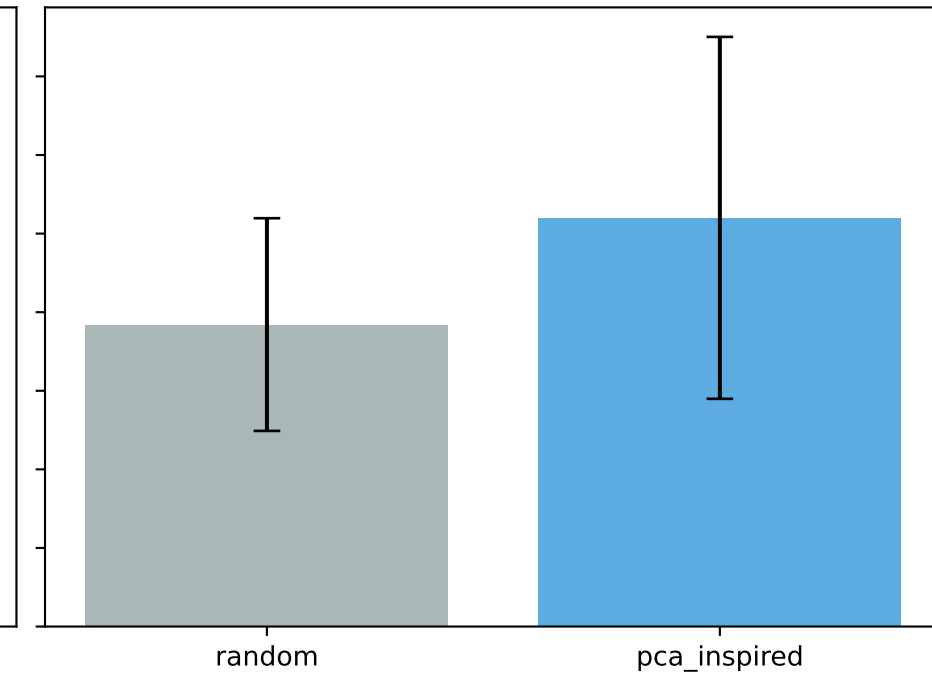
Multi-Lag Fidelity
