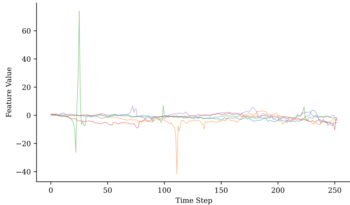
Geometric SDE Paths (dim 1)
