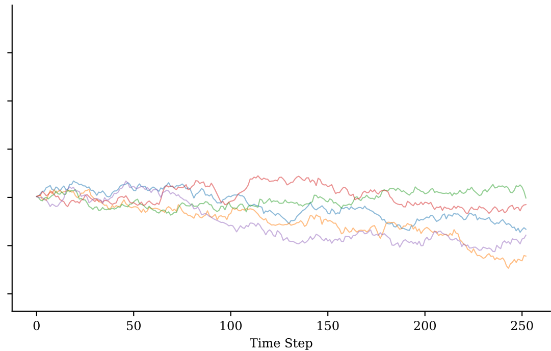
Standard SDE Paths (dim 1)
