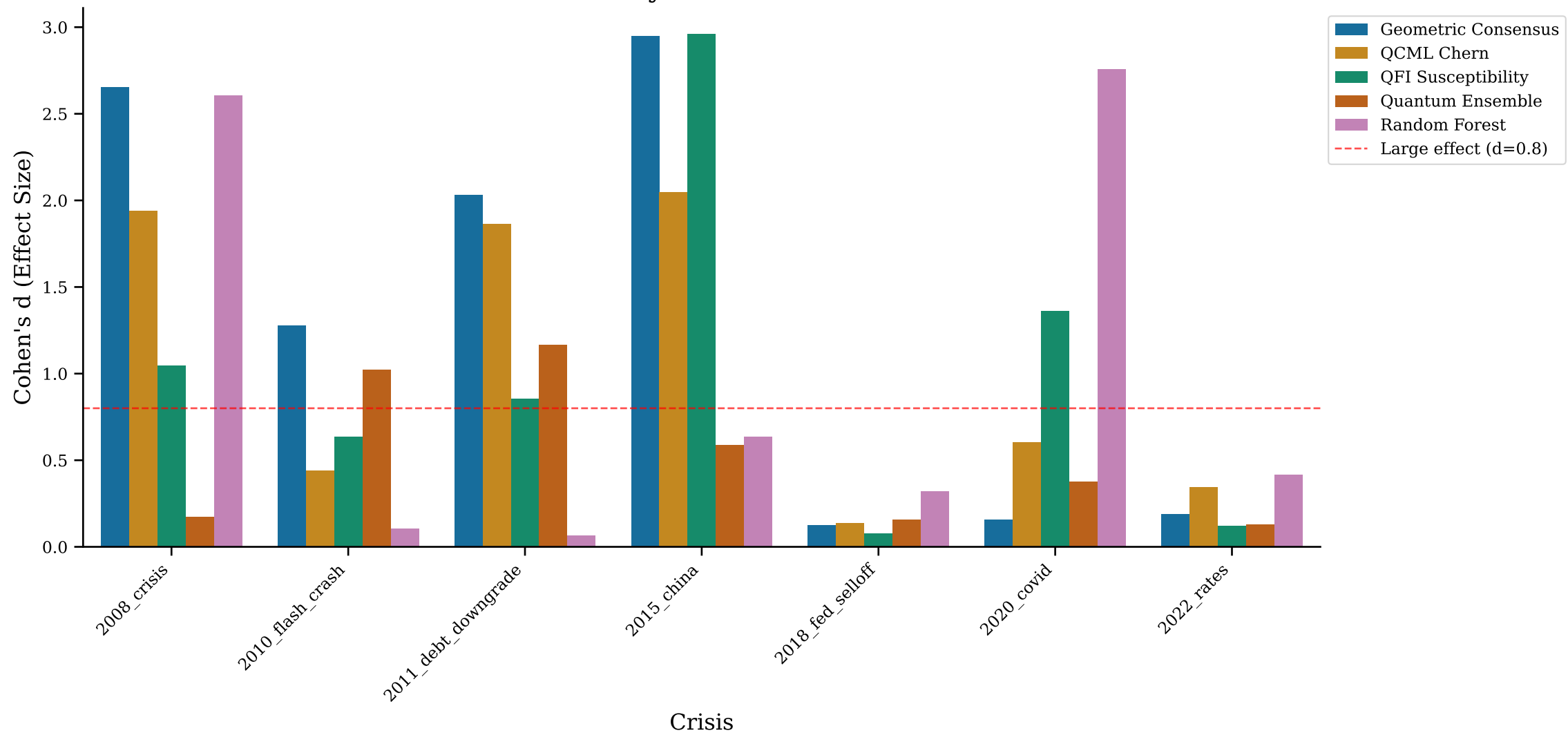
Effect Size by Crisis and Method
