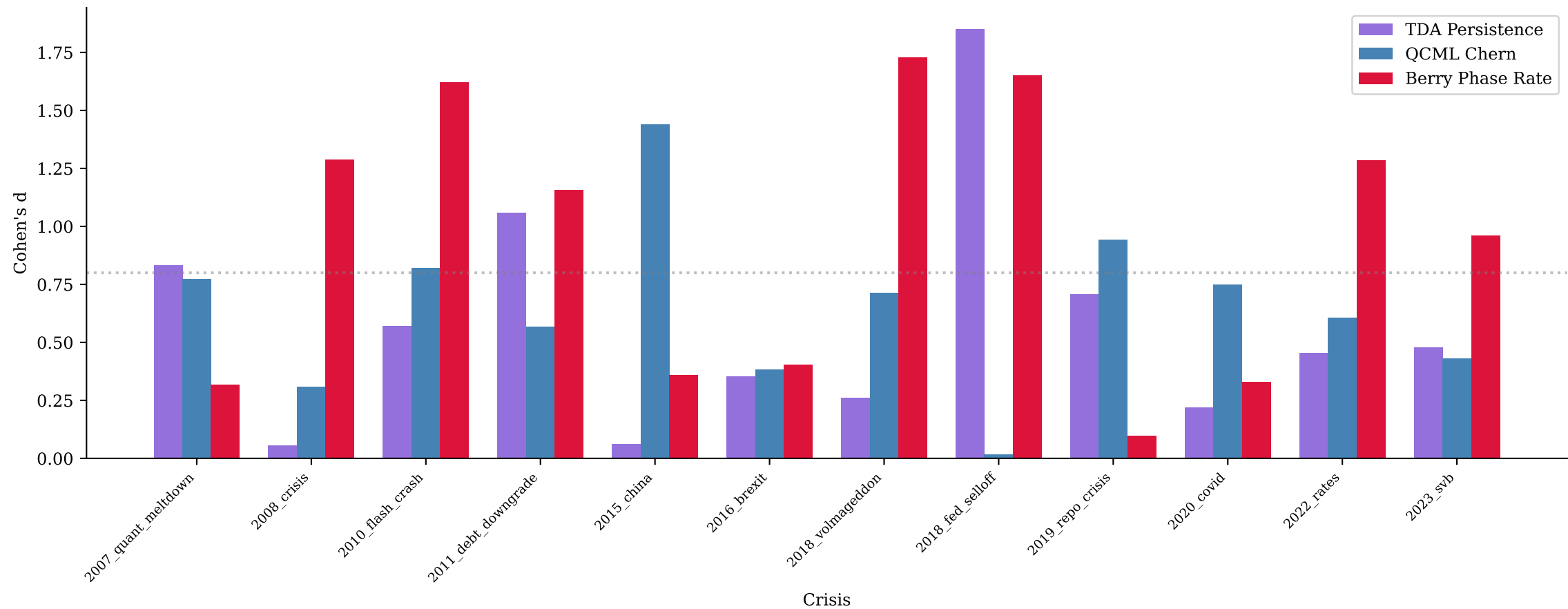
TDA vs QCML: Crisis Detection Effect Sizes
