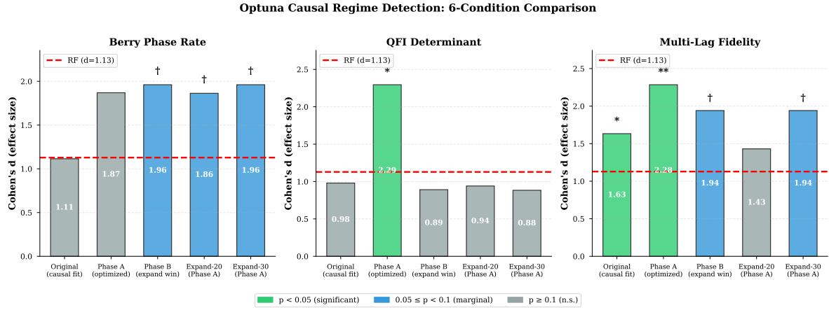
Figure 1: Causal optimization: mean Cohen's d across 12 crises under six conditions. Stars: **p < 0.01 , *p < 0.05 , †p < 0.1 vs. RF. QFI and Multi-Lag (Phase A) significantly beat RF.
