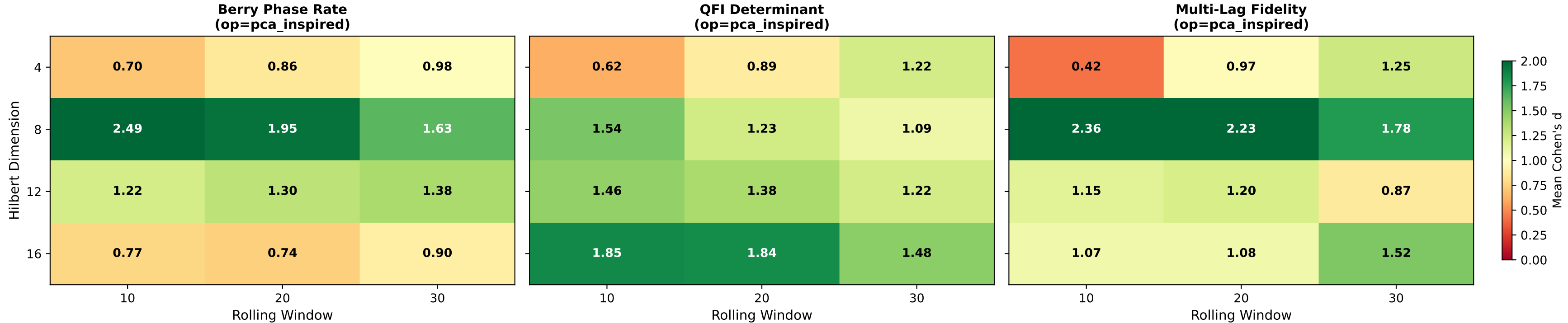
Extended Sensitivity: Hilbert Dim x Rolling Window (Best PCA, Best Op)
