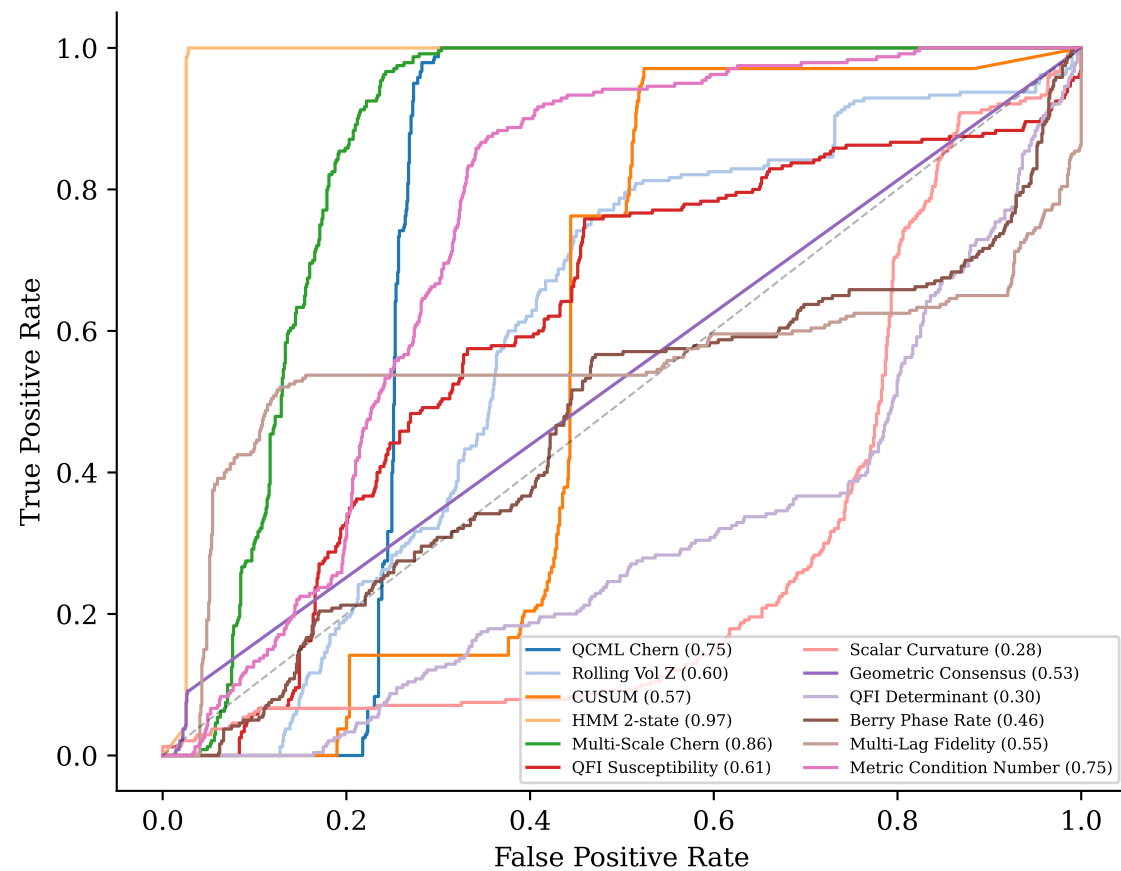
ROC Curves: Crisis Detection vs. Calm Periods
