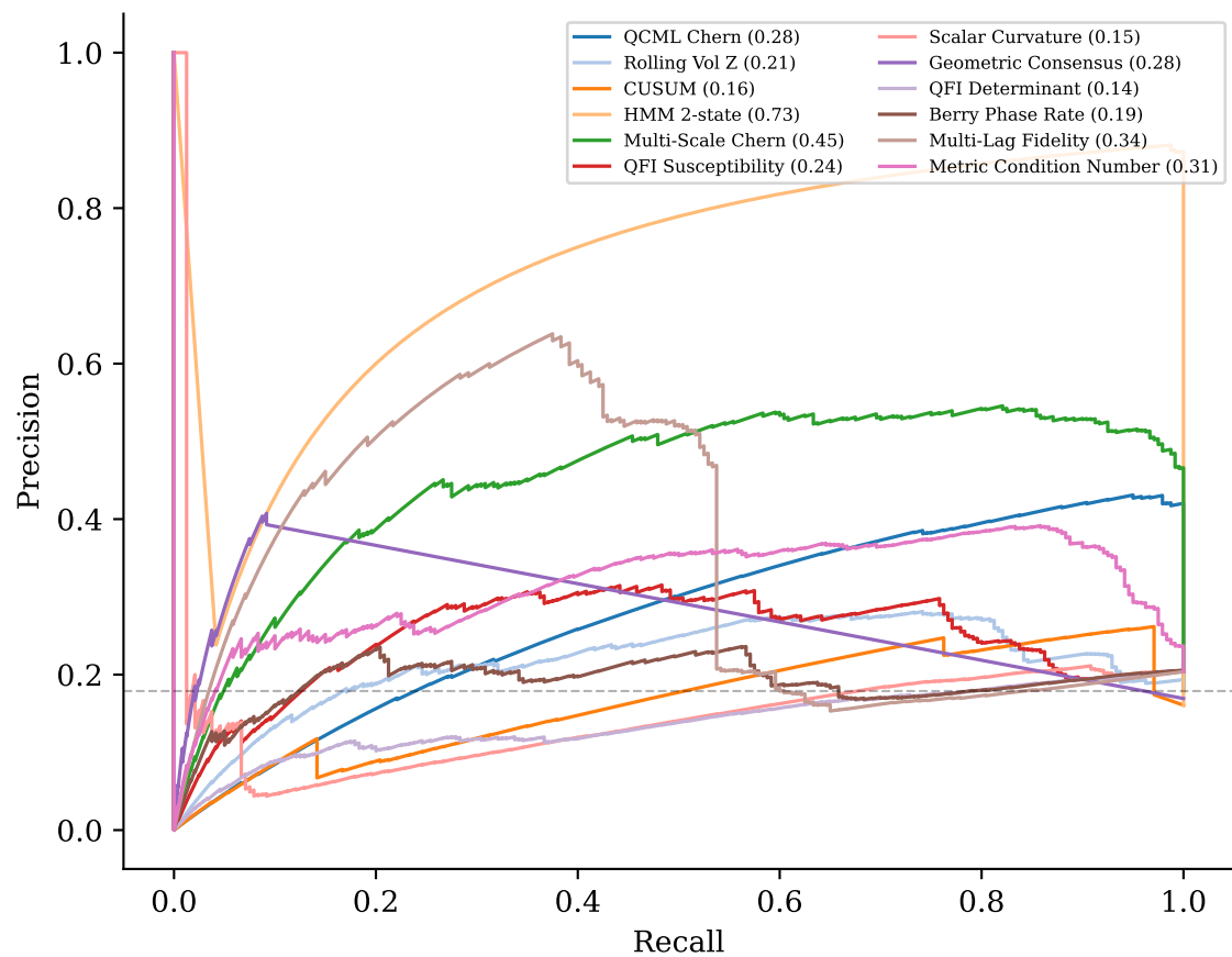
Precision-Recall Curves
