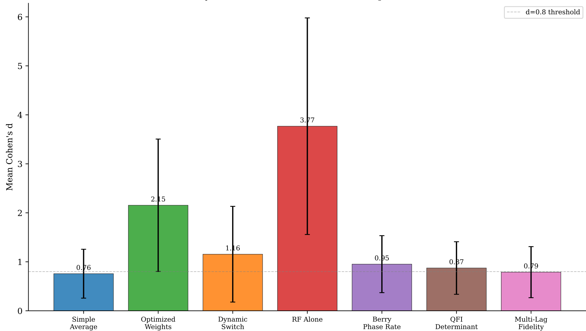
Hybrid Ensemble vs Individual Components
