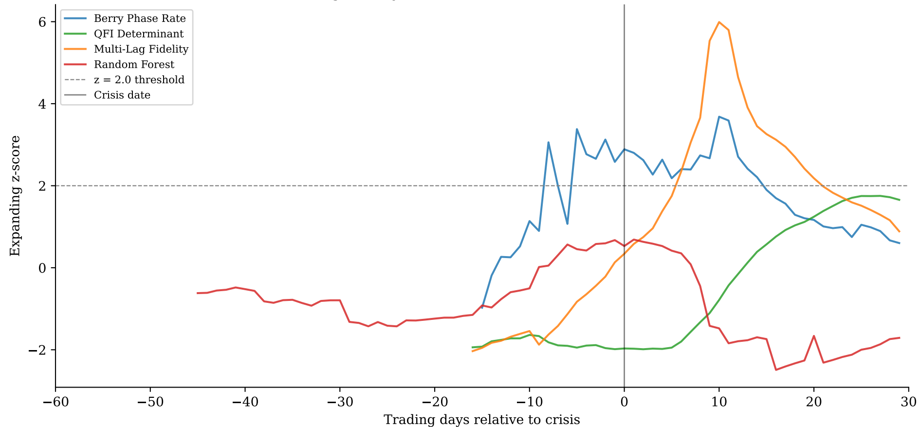
Signal trajectories: 2007 Quant Meltdown
