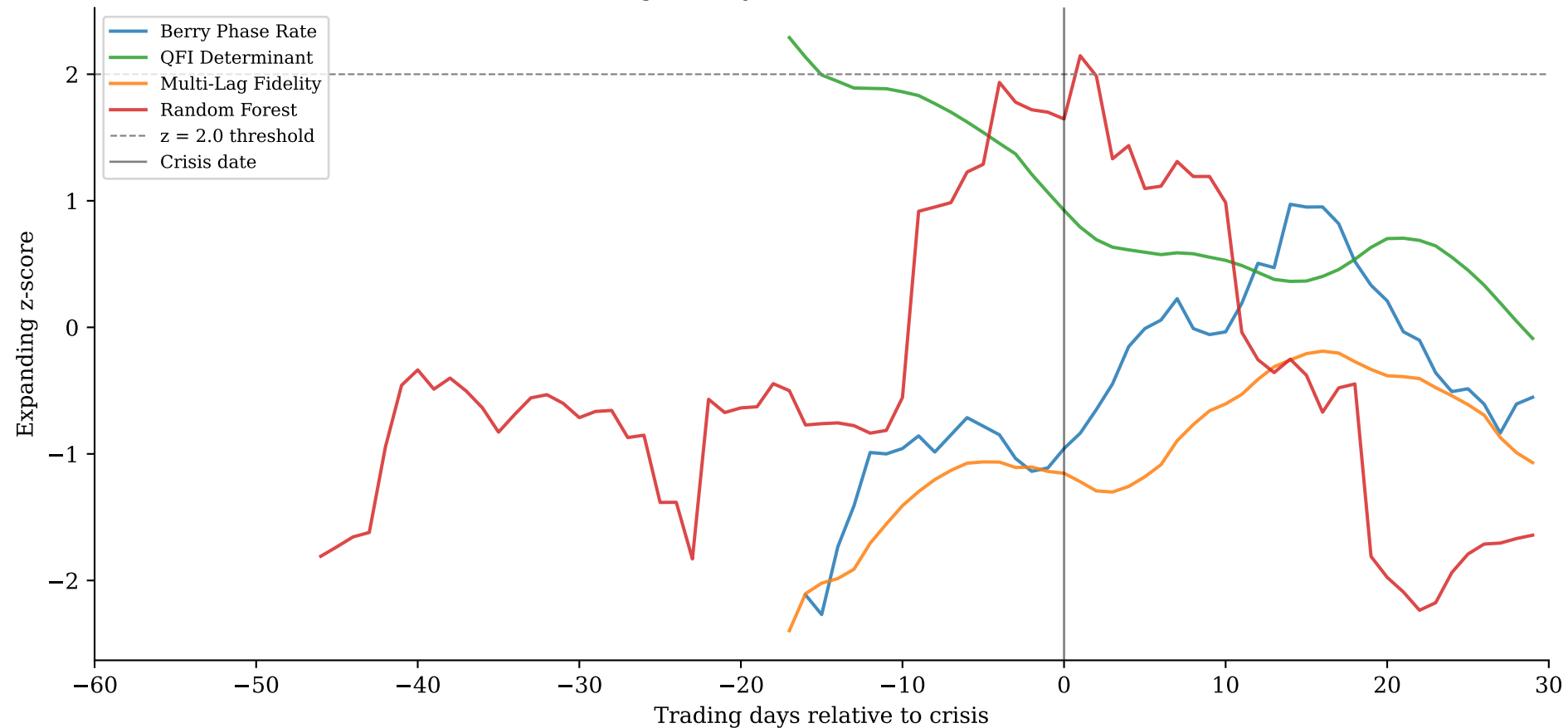
Signal trajectories: 2008 Crisis
