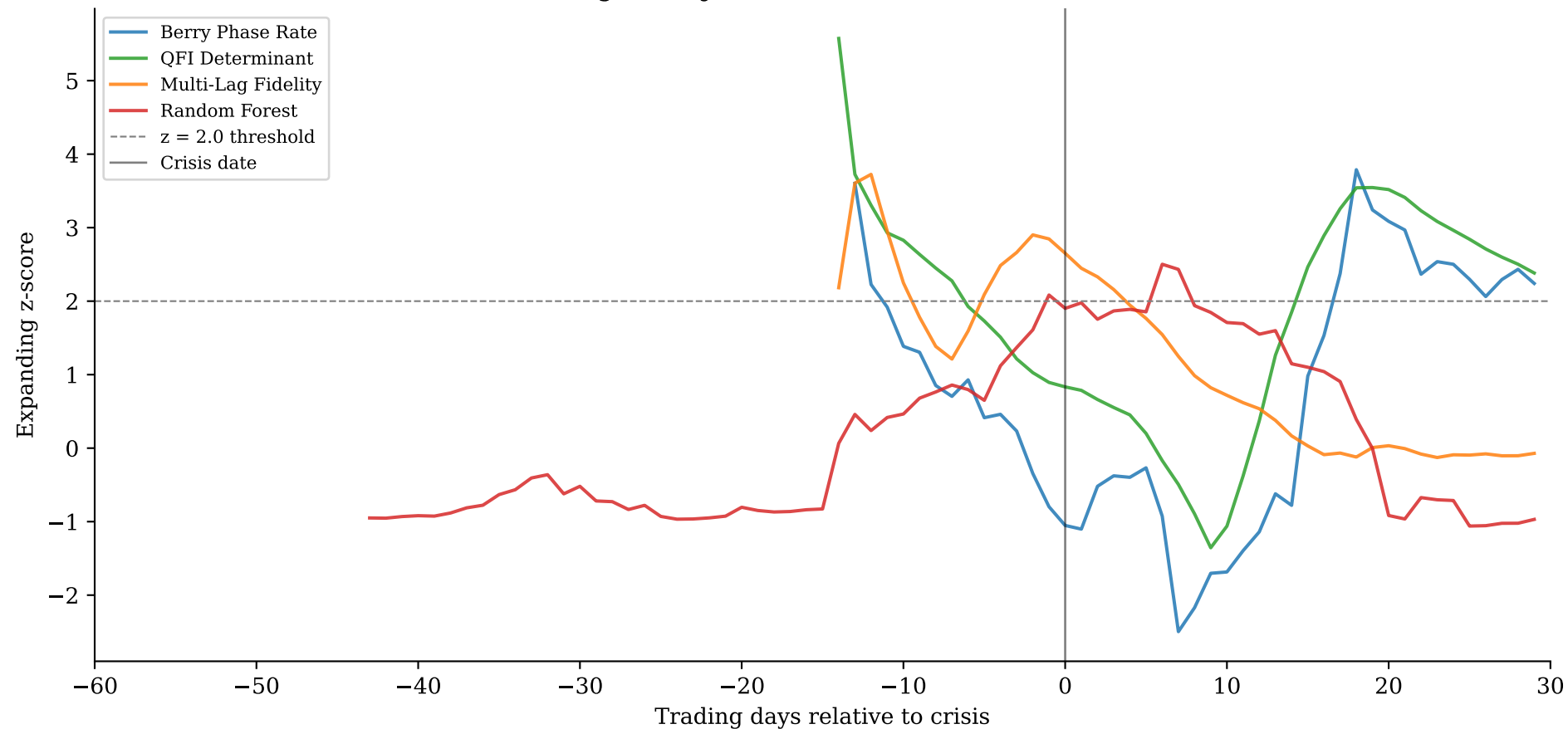
Signal trajectories: 2010 Flash Crash
